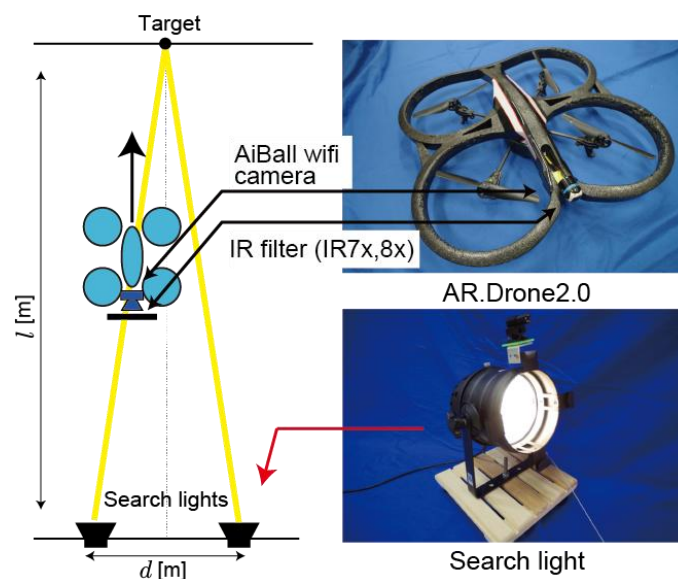
FIGURE 2. Basic concept of 50 m range position measurement method of the autonomous flight device. Two searchlights (Stage Evolution, PAR56SBG) were used for the position measurement of the drone in the space
