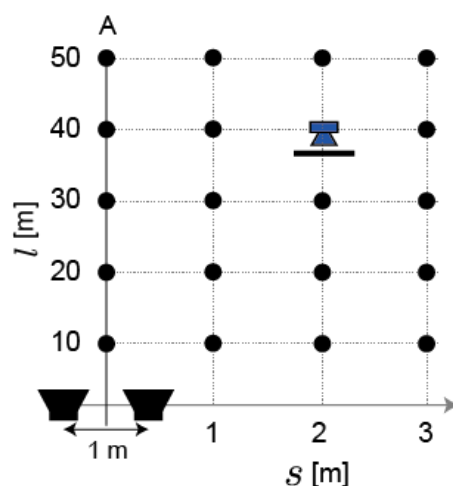
FIGURE 5. Experiment 4 setup of the 3 m×50 m range position / distance detectability measurement in outdoor situation.
