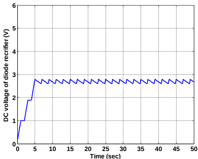
FIGURE 5: DC voltage of the diode rectifier
