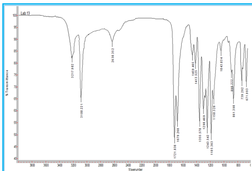
FIGURE 1 . IR SPECTRA OF POLYAMIDOSULFOIMIDES ON THE BASIS OF DICHLOROANHYDRIDES OF SACCHARIN-5-CARBOXYLIC ACID AND ALIPHATIC DIAMINES
