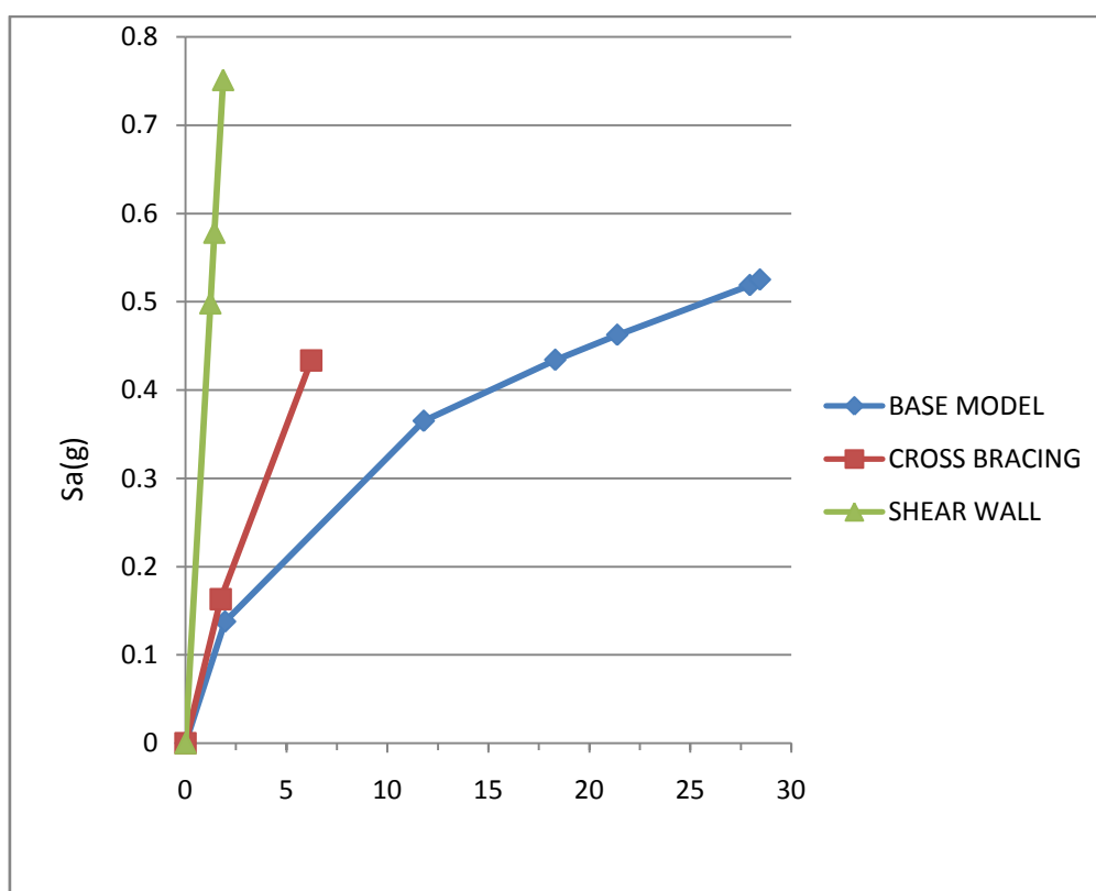
FIGURE 6.12: Capacity Spectrum
