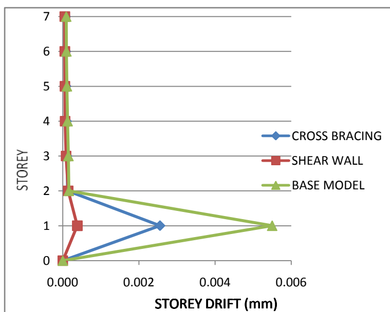
FIGURE 6.5- Observed values of Storey Drifts for North Ridge
