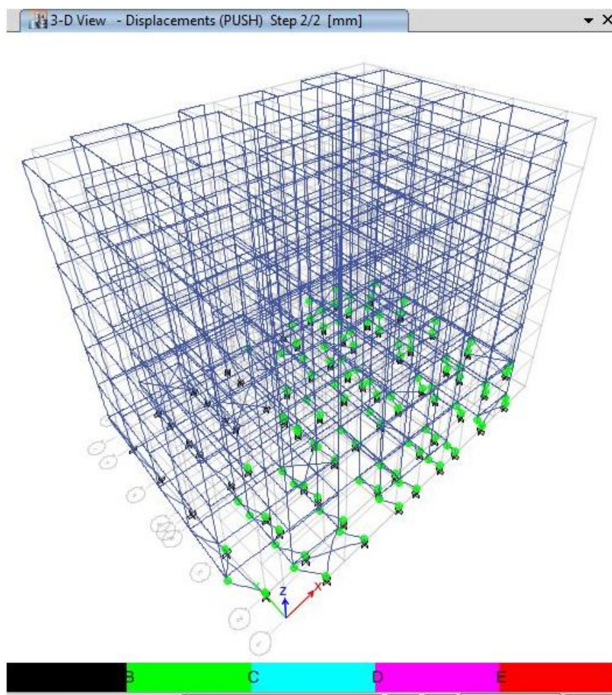
FIGURE 6.15: Hinge failure pattern for model retrofitted by cross bracing
