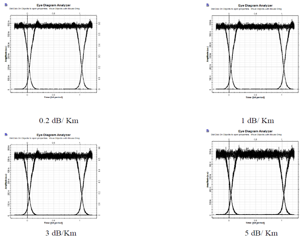
FIG. 4: EYE DIAGRAM ANALYZER FOR DIFFERENT ATTENUATION
