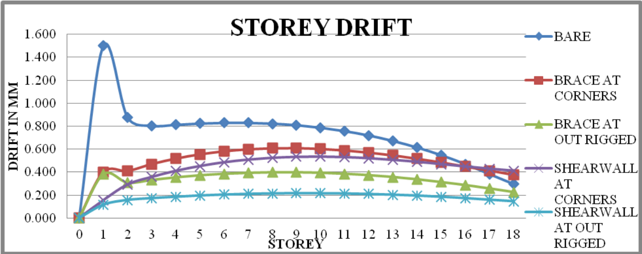
GRAPH.6. PLOT OF STOREY DRIFT OF G+18 T SHAPE SOFT STOREY BUILDING
