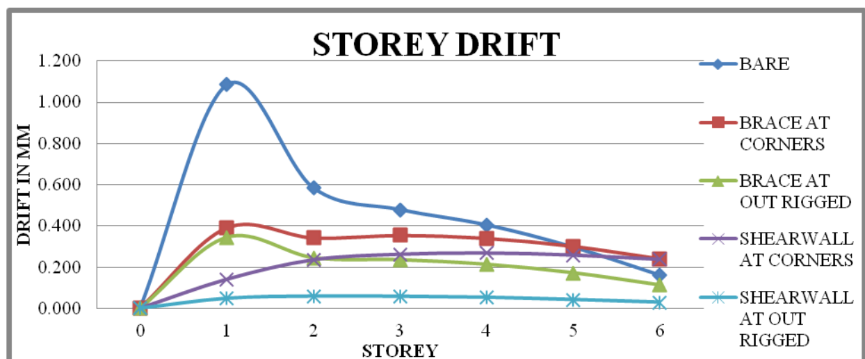
GRAPH.2. PLOT OF STOREY DRIFT OF G+6 T SHAPE SOFT STOREY BUILDING
