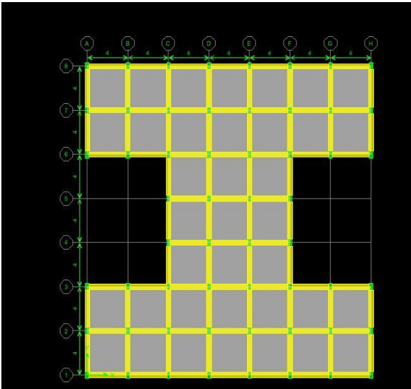
FIG.2. I SHAPE BUILDING
