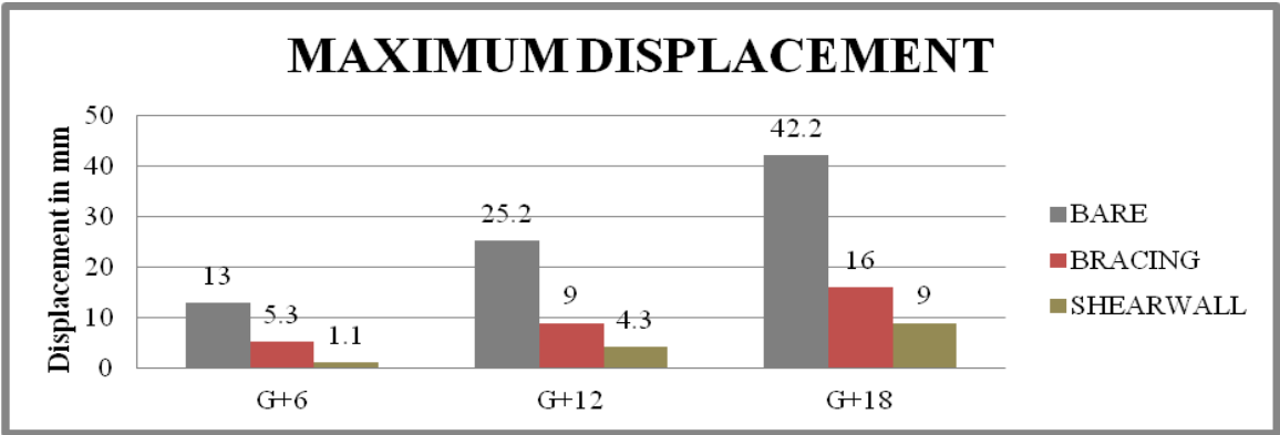
GRAPH.8. PLOT OF MAXIMUM REDUCED DISPLACEMENT OF T SHAPE SOFT STOREY BUILDING
