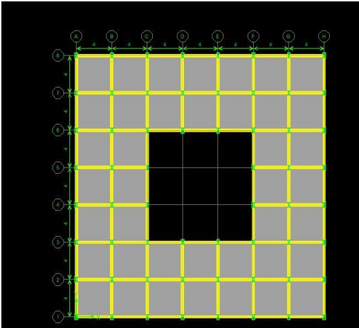
FIG.4. DIAPHRAGM OPENING
