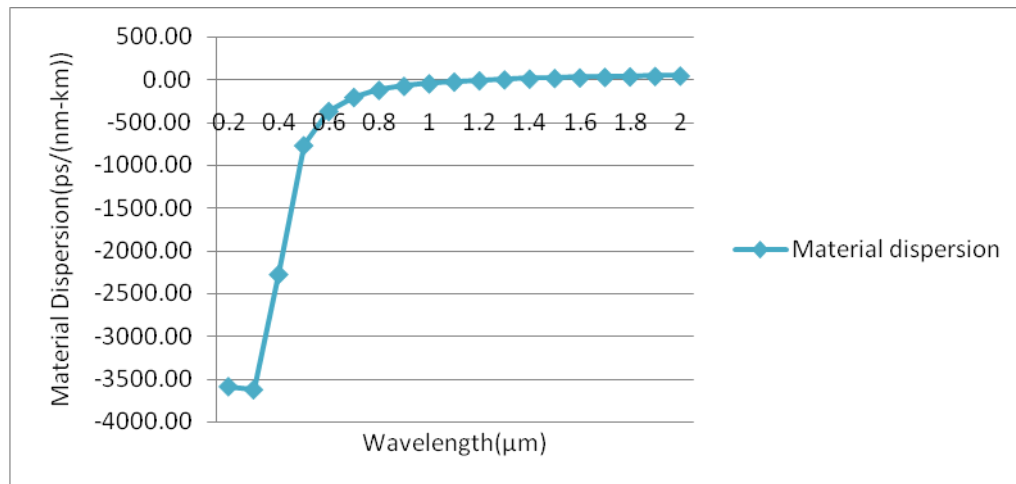
FIG. 3 MATERIAL DISPERSION OF FUSED SILICA GLASS
