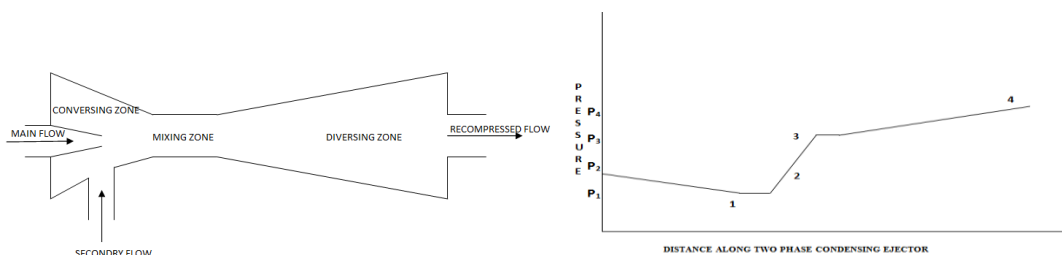
Fig 2,3: pressure variation along the condensing ejector
