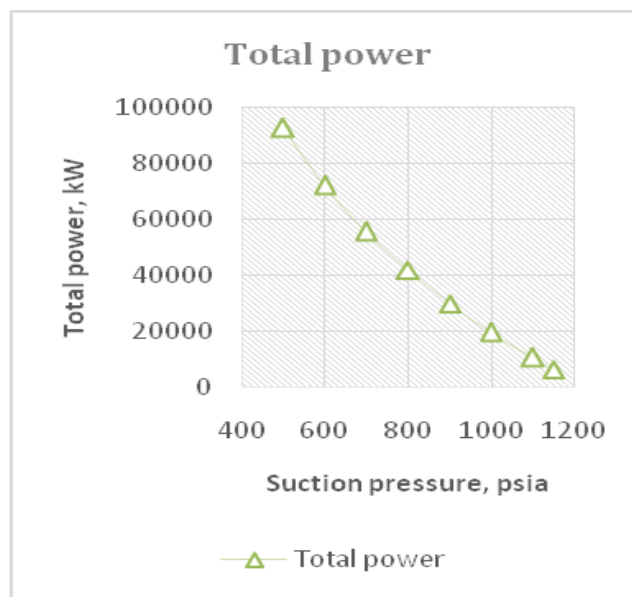
FIGURE V.2 SUCTION PRESSURE VS TOTAL
