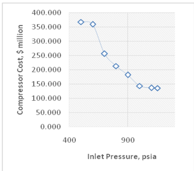
FIGURE V.1 INLET PRESSURE VS COMPRESSOR COST
