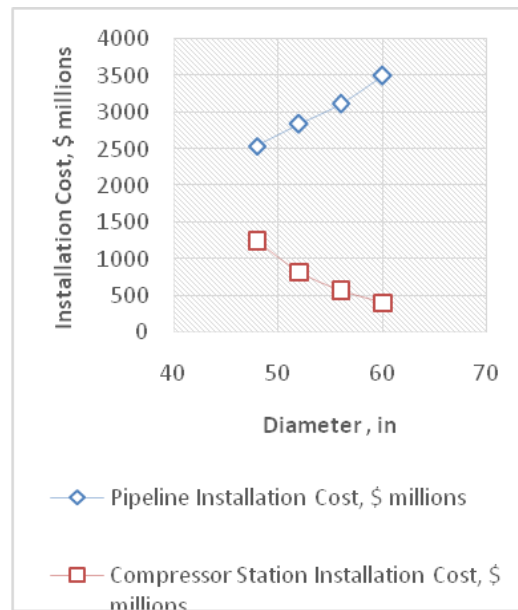
FIGURE V.4 PIPE DIAMETER VS. INSTALLATION
