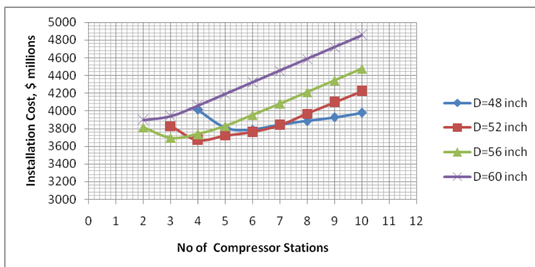
FIGURE .V.6 NUMBER OF COMPRESSOR STATIONS VS INSTALLATION COST
