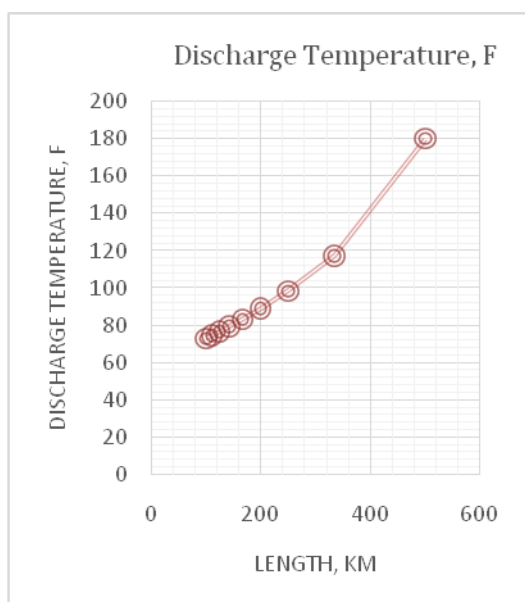
FIGURE 5.3 COMPRESSOR DISCHARGE TEMPERATURE
