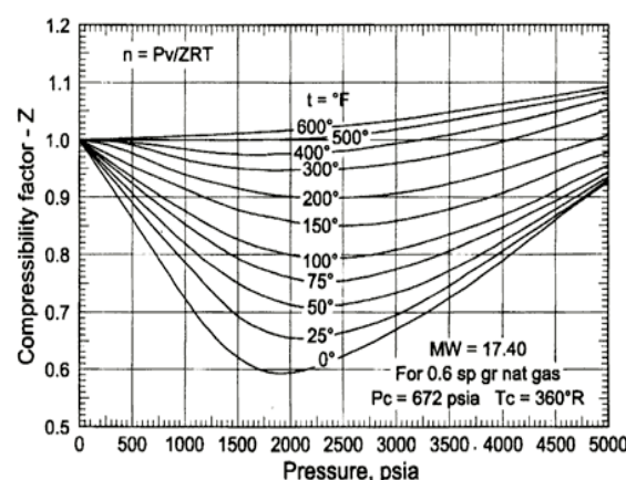
FIGURE 2. COMPRESSIBILITY FACTOR GRAPH[14]
