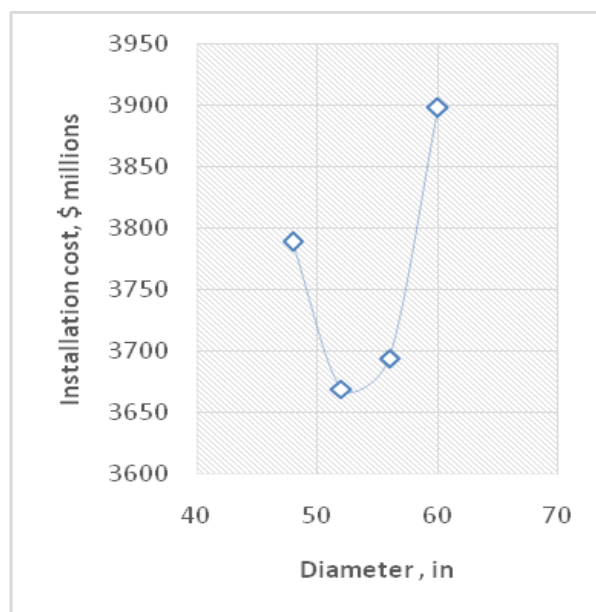
FIGURE 5.5: TOTAL MINIMUM INSTALLATION COST
