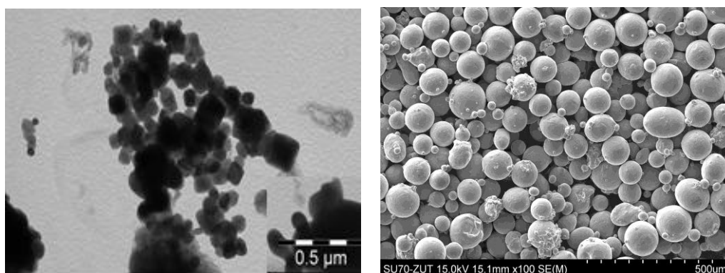
FIGURE 1: (A) TEM IMAGE OF NC-TiC, (B) SEM IMAGE OF Ti POWDER.
