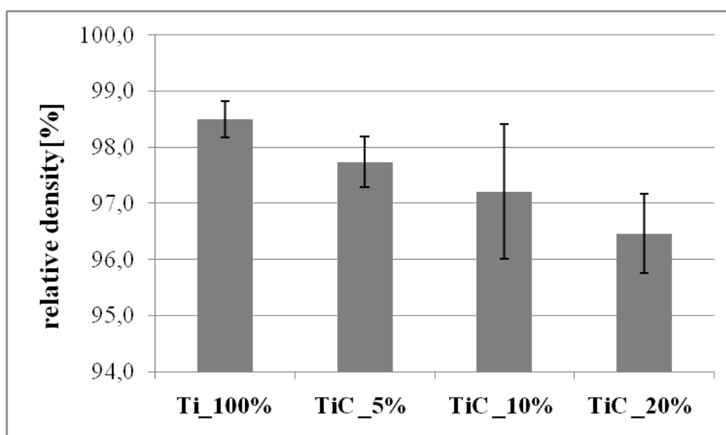
FIGURE 3: DEPENDENCE OF THE RELATIVE DENSITY ON TiC CONTENT
