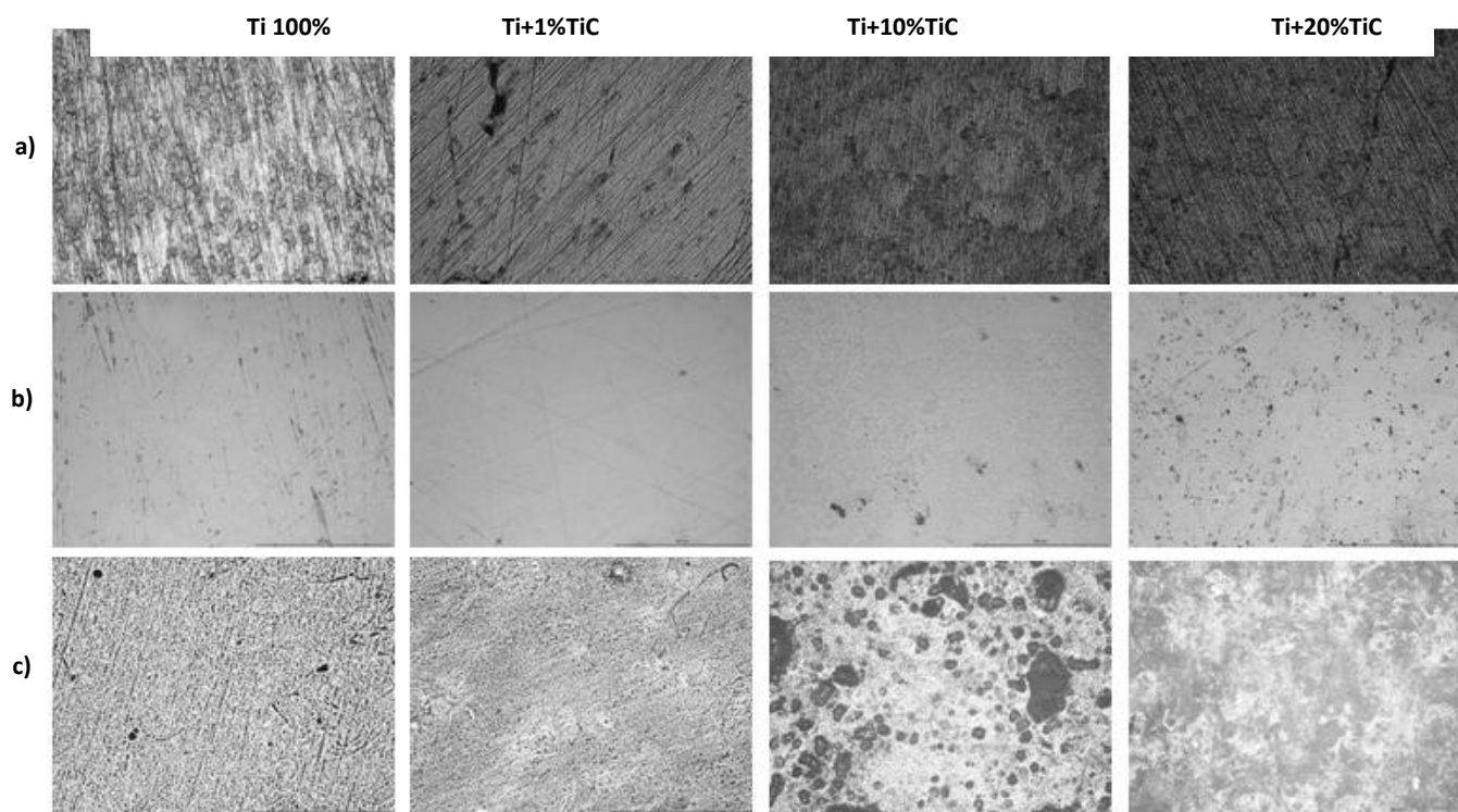
FIGURE 4: THE SURFACE OF THE Ti 100%, (Ti 99%+TiC 1%), (Ti 90% + TiC 10%), (Ti 80% + TiC 20%) SAMPLES AFTER (A) GRINDING, (B) POLISHING, (C) ELECTROPOLISHING; X 100
