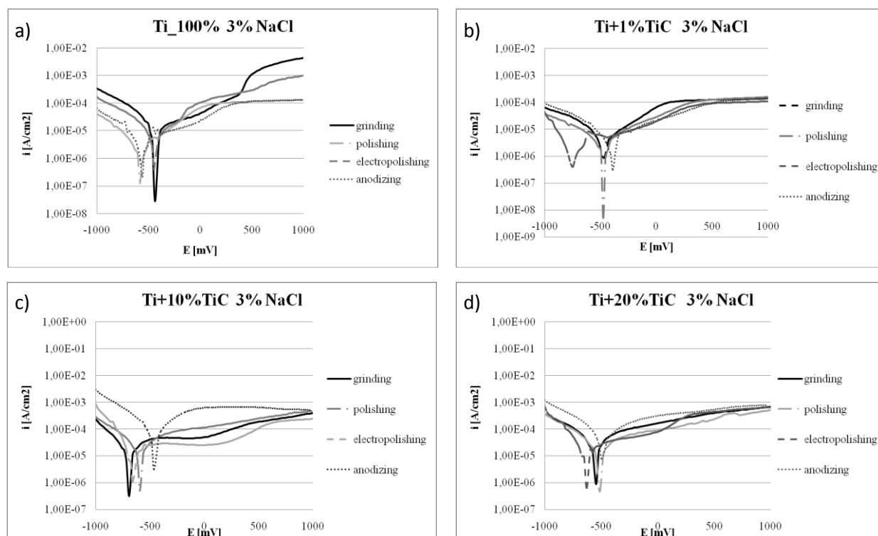
FIGURE 5: EXPERIMENTAL POLARIZATION CURVES FOR TiC/Ti NANOCOMPOSITES IN 3 WT% SOLUTION OF NaCl AT ROOM TEMPERATURE AFTER POLISHING, GRINDING, ELECTROPOLISHING AND ANODIZING; (A) Ti 100%, (B) Ti 99%+TiC 1%, (C) Ti 90% + TiC 10%, (D) Ti 80% + TiC 20%
