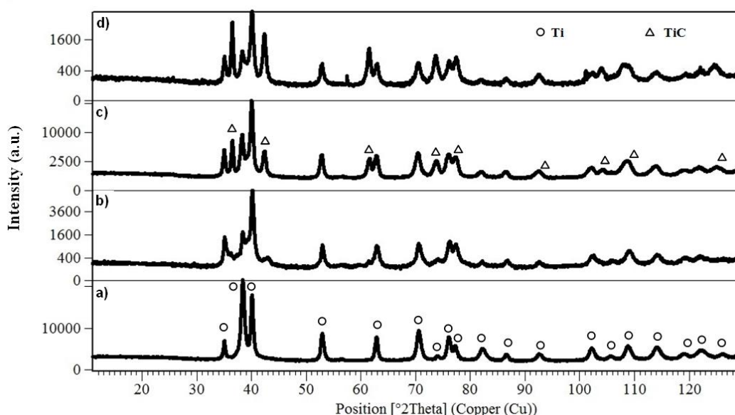
FIGURE 2: COMPARISON OF THE XRD PATTERNS OF NC-TiC POWDER AND TiC/Ti NANOCOMPOSITES CONTAINING RESPECTIVELY 1, 10 AND 20 VOL% NC-TiC IN Ti MATRIX
