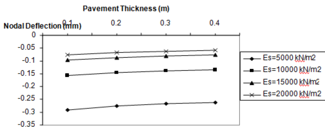
FIG. 6: DESIGN CHART, PRESSURE=100 kN/m 2
