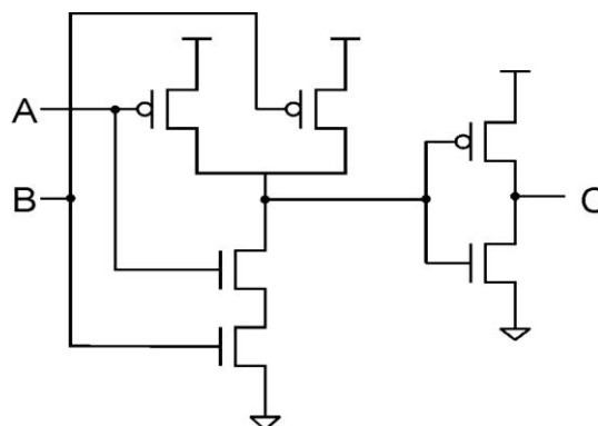
FIG.1 SCHEMATIC DIAGRAM OF CSL AND GATE
