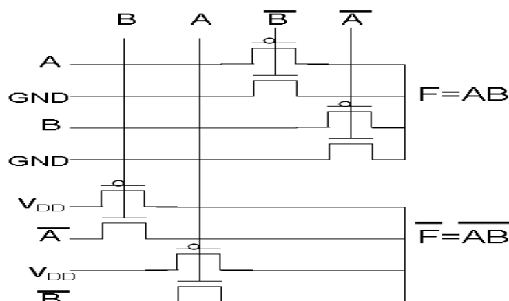
FIG. 5 SCHEMATIC DIAGRAM OF DPL AND GATE
