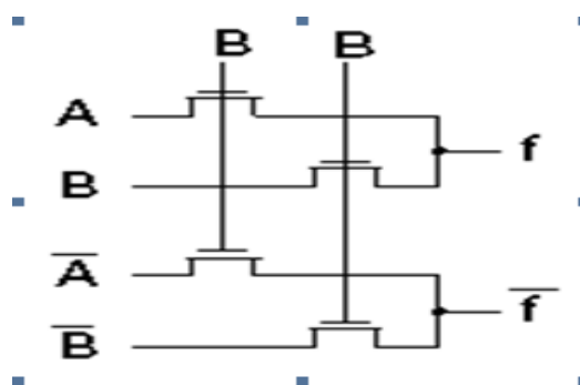
FIG. 4 SCHEMATIC DIAGRAM OF CPL AND GATE
