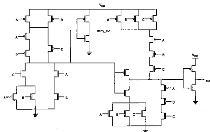
FIG. 2 SCHEMATIC DIAGRAM OF CSL FULL ADDER
