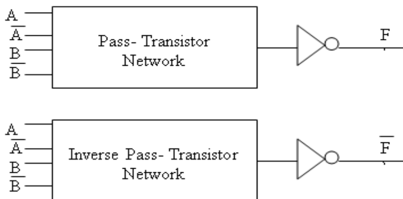
FIG.3 BASIC CONCEPT OF CPL
