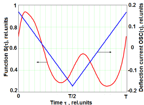
FIG.24RECORDING OF DEFLECTION COILS CURRENT SIGNAL OSC(\tau) AND FUNCTION S(\tau) OBTAINED USING THE COHERENT ACCUMULATION METHOD DURING STEEL WELDING WITH OSCILLATION ALONG THE JOINT ( P=3 kW, BEAM CURRENT 50 mA, OSCILLATION FREQUENCY f=630 Hz, OSCILLATIONS SWEEP SIZE 2A=1.5 mm)[75]
