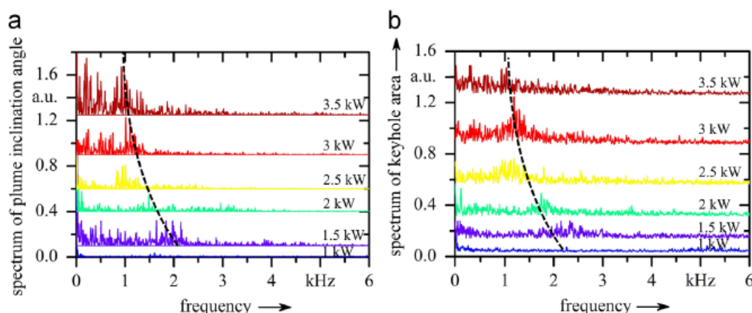
FIG.11. SPECTRA OF THE PLUME INCLINATION ANGLE (A) AND THE VISIBLE KEYHOLE AREA (B) FOR A CONSTANT FEED RATE OF 7 M/MIN ON ONE 5 MM STAINLESS STEEL PLATE. THE SPECTRA ARE PLOTTED TO SEPARATE THEM BEST, THE DASHED LINE INDICATES THE TREND OF THE DOMINATING FREQUENCIES (NO DOMINATING FREQUENCY VISIBLE FOR 1 kW).
