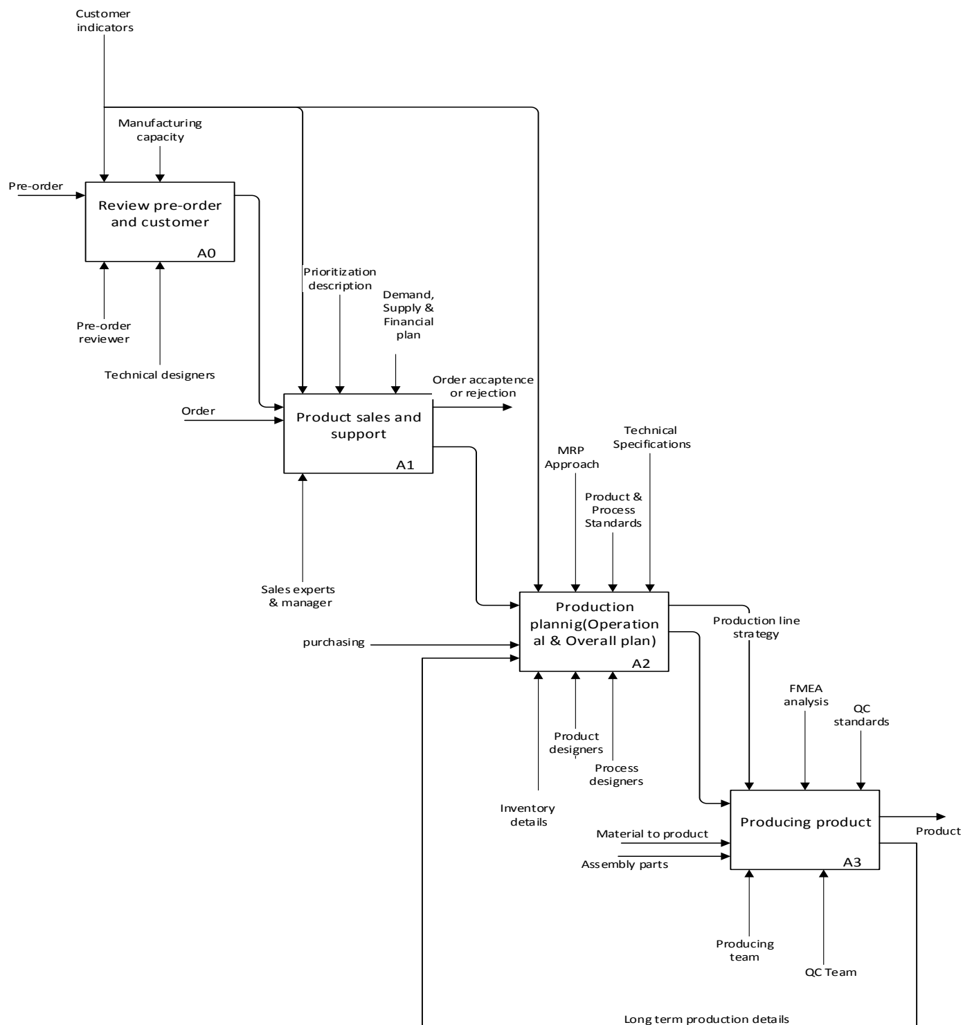
FIG. 1: FOUR GENERAL PROCESSES LEVEL-0 IDEF0 MODEL
