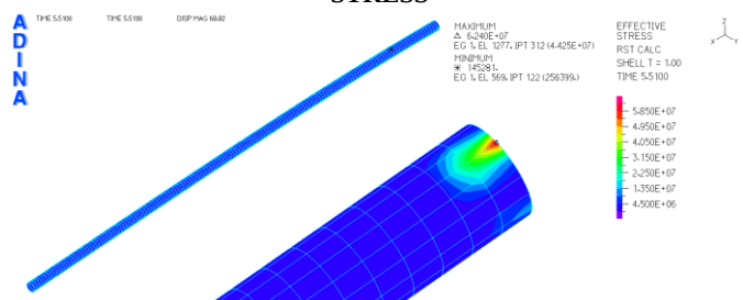
FIG.5 WALL THICKNESS IS 28.7MM EQUIVALENT STRESS
