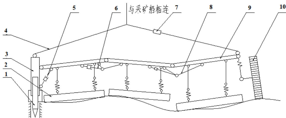
FIG.1 CANTILEVER - OUTRIGGER COMPOSITE MINING MECHANISM
