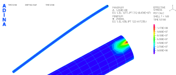
FIG.2 WALL THICKNESS IS 9.5MM EQUIVALENT STRESS
