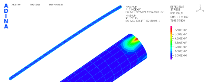
FIG.3 WALL THICKNESS IS 16.9MM EQUIVALENT STRESS
