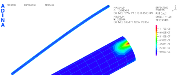
FIG.4 WALL THICKNESS IS 16.9MM EQUIVALENT STRESS
