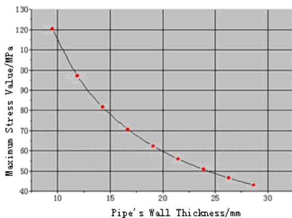
FIG.6 MAXIMUM STRESS OF DIFFERENT WALL THICKNESS
