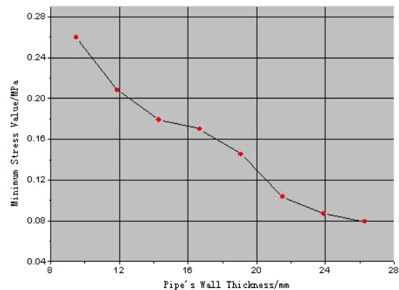
FIG.7 MINIMUM STRESS OF DIFFERENT WALL THICKNESS
