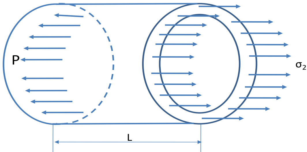
FIGURE 4: Stress and pressure acting on a thin walled cylinder when cut by a plane perpendicular to the axis of the cylinder
