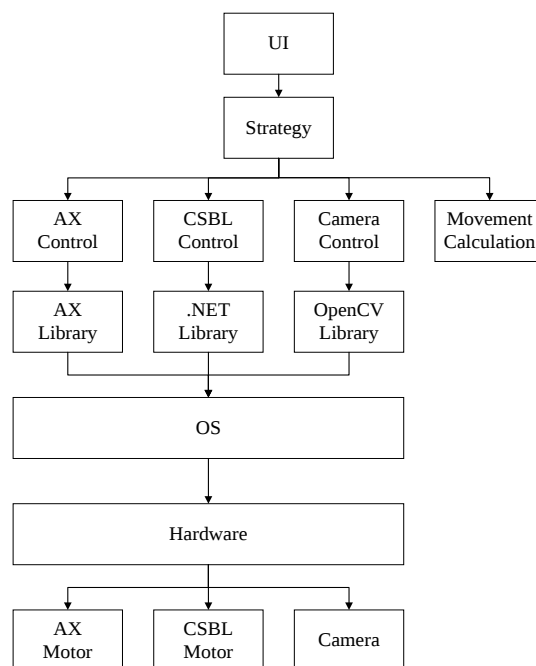
FIG. 1. THE ARCHITECTURE OF SOFTWARE SYSTEM.
