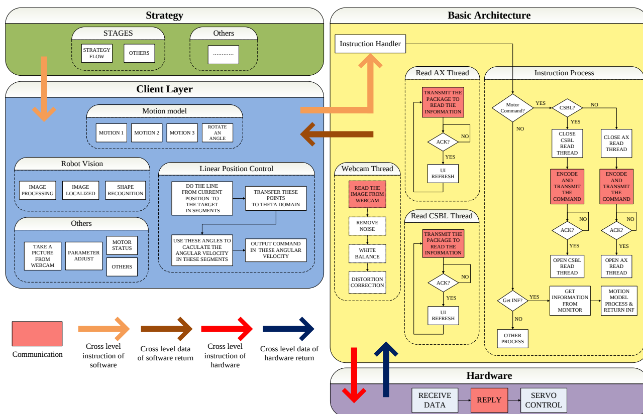
FIG. 1. THE ARCHITECTURE OF SOFTWARE SYSTEM.
