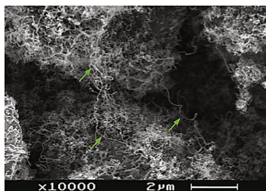
FIG. 5. SEM IMAGES OF CNFs GROWN ON CLINKER. [17].
