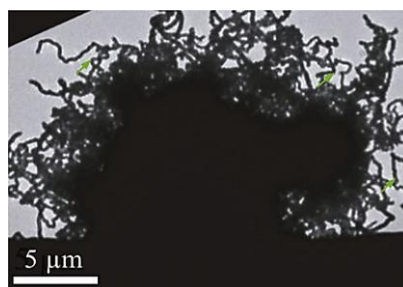
FIG. 2. TEM IMAGE OF COMPLETE COVERAGE OF THE CEMENT PARTICLES BY CNTs/CNFs [14].
