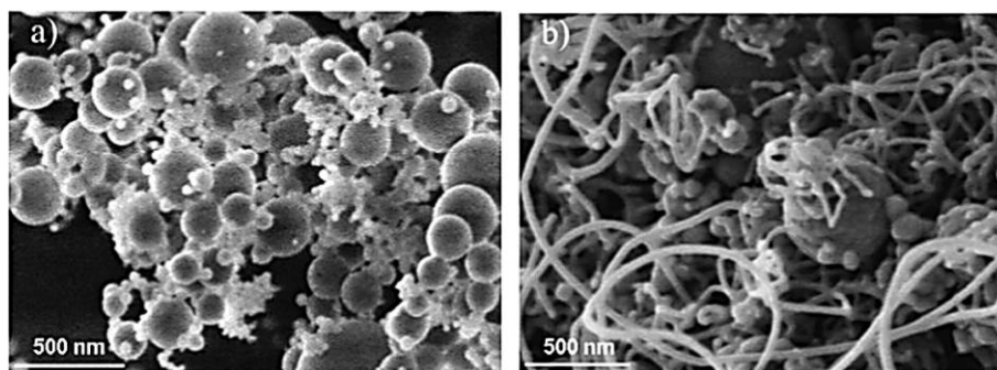
FIG. 3. SEM IMAGES OF (A) PRISTINE SILICA PARTICLES AND (B) CNTS GROWN ON THE SURFACE OF SILICA [12].
