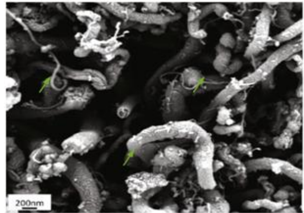
FIG. 7. SEM IMAGES OF CNTs AND CNFs GROWN ON FLY ASH[23].
