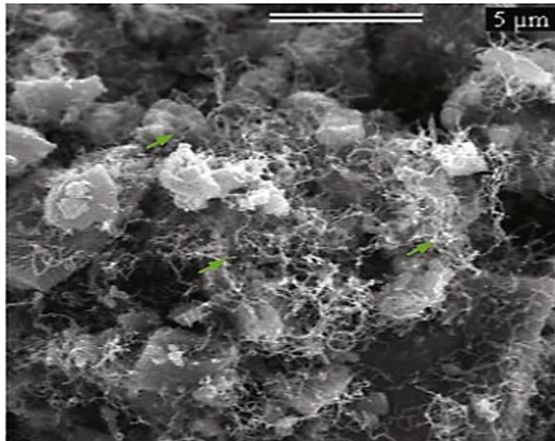
FIG. 6. SEM IMAGE OF CNTs GROWN ON CLINKER[21].
