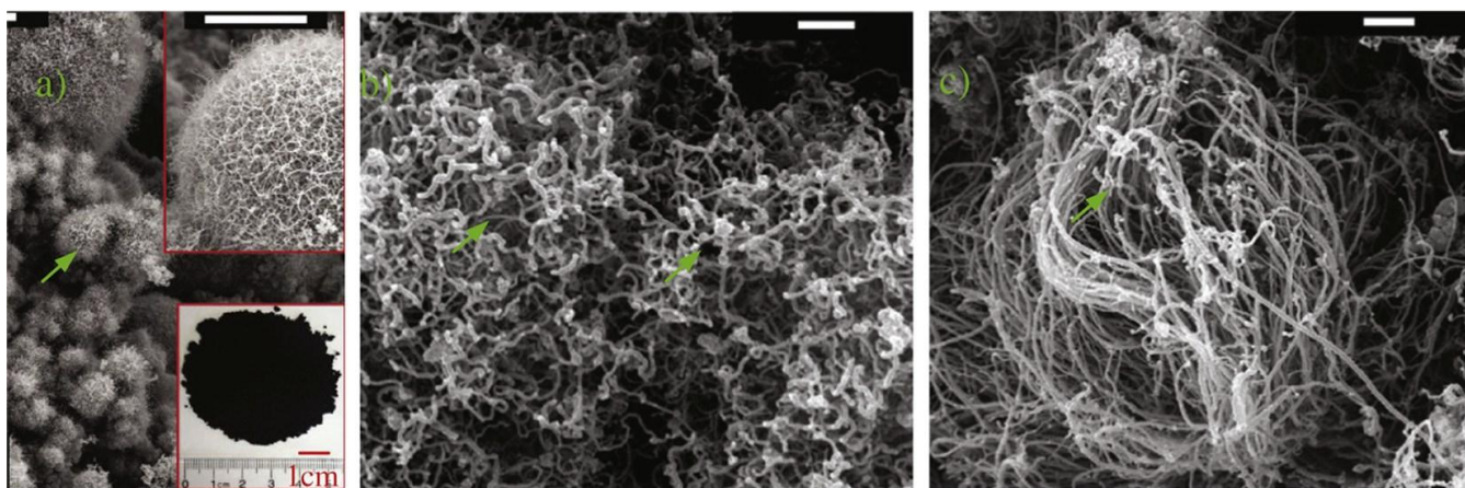
FIG. 9. (A) SEM IMAGES OF THE AS-PRODUCED CNTs ON FLY ASH, INSETS: (TOP) ZOOM-IN SEM IMAGE; (BOTTOM) DIGITAL PICTURE OF COATED FLY ASH (B AND C) SEM IMAGES OF CNTs COATED POLYPYRROLE COATED FLY ASH [24–26].
