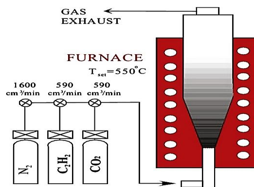
FIG. 4. SCHEMATIC PRESENTATION OF THE FLUIDIZED BED REACTOR USED FOR SYNTHESIS OF CNFs ON THE SURFACE OF CLINKER PARTICLES [17].
