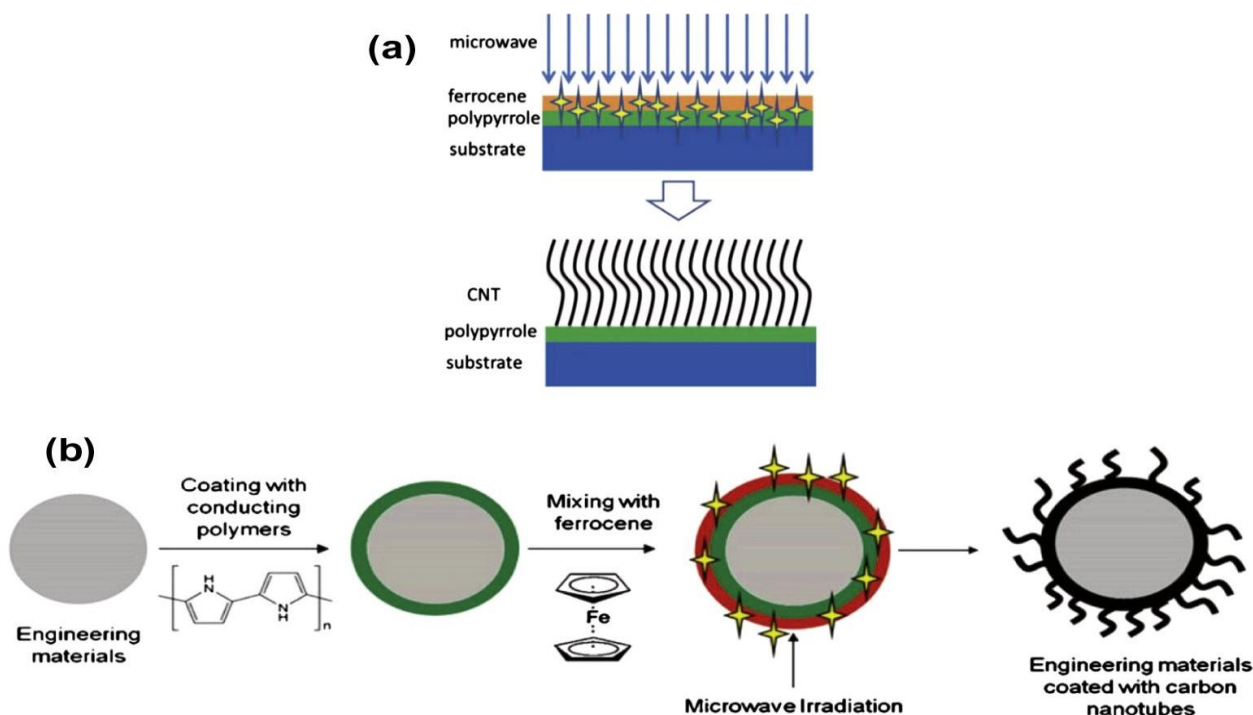
FIG. 8. (A) MICROWAVE INITIATED CNTs GROWTH ON CONDUCTIVE SURFACES AND (B) MICROWAVE INITIATED CNTs GROWTH ON ENGINEERING MATERIALS [24–26].
