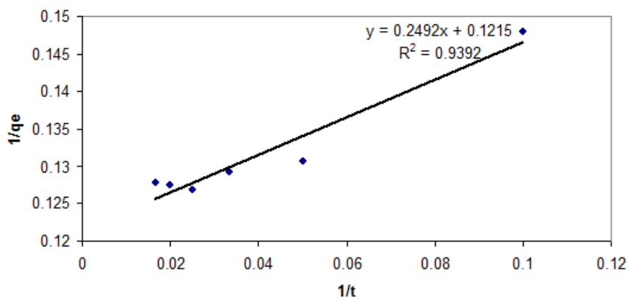
FIGURE 4: PSEUDO-SECOND ORDER KINETIC MODEL FOR RE-REFINING OF WASTE LUBRICATING OIL USING ACTIVATED UKPOR CLAY (FOR EQUATION 3)
