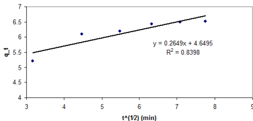
FIGURE 7: INTRA PARTICLE DIFFUSION KINETIC MODEL FOR RE-REFINING OF WASTE LUBRICATING OIL USING ACTIVATED UKPOR CLAY
