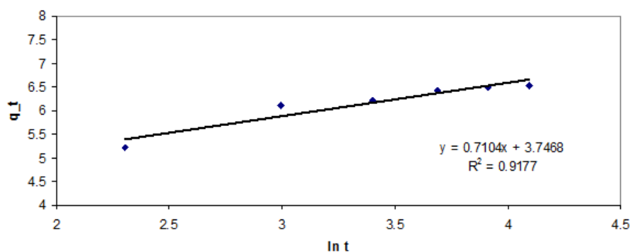
FIGURE 8: ELOVICH KINETIC MODEL FOR RE-REFINING OF WASTE LUBRICATING OIL USING ACTIVATED UKPOR CLAY
