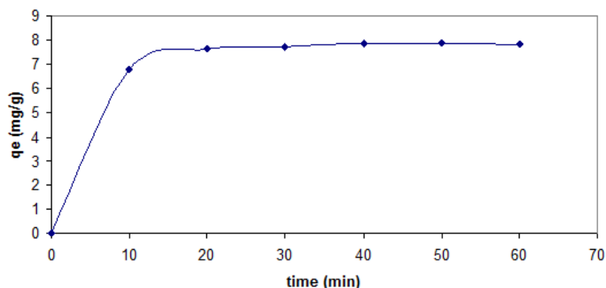
FIGURE 2: EFFECT OF CONTACT TIME ON THE ADSORPTION TREATMENT OF WASTE LUBRICATING OIL USING ACTIVATED UKPOR CLAY
