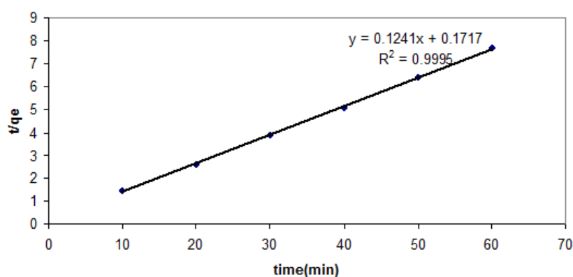
FIGURE 5: PSEUDO-SECOND ORDER KINETIC MODEL FOR RE-REFINING OF WASTE LUBRICATING OIL USING ACTIVATED UKPOR CLAY (EQUATION 4)
