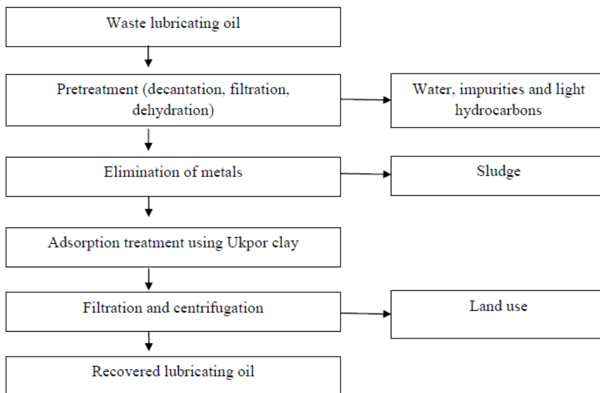
FIGURE 1: SCHEMATIC DIAGRAM OF WASTE LUBRICATING OIL RE-REFINING PROCESS USING ACTIVATED UKPOR CLAY.
