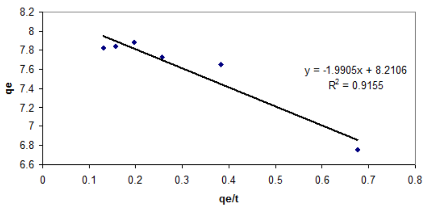
FIGURE 6: PSEUDO-SECOND ORDER KINETIC MODEL FOR RE-RECYCLING OF WASTE LUBRICATING OIL USING ACTIVATED UKPOR CLAY (EQUATION 5)
