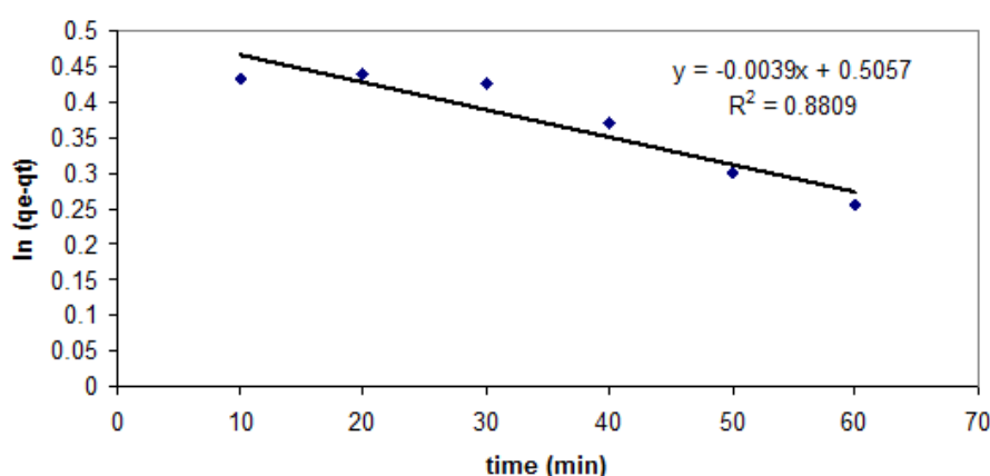
FIGURE 3: PSEUDO-FIRST ORDER KINETIC MODEL FOR RE-REFINING OF WASTE LUBRICATING OIL USING ACTIVATED UKPOR CLAY
