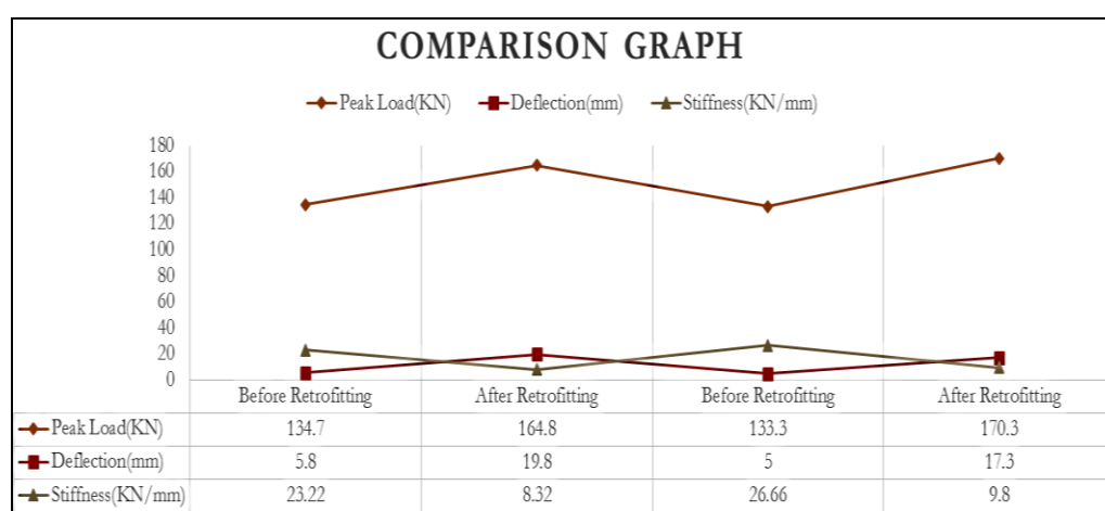
GRAPH 3: COMPARISON FOR FLEXURAL SPECIMEN (BEFORE AND AFTER RETROFITTING)
