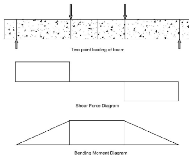
FIG 7 SHEAR FORCE AND BENDING MOMENT DIAGRAM FOR TWO POINT LOADING
