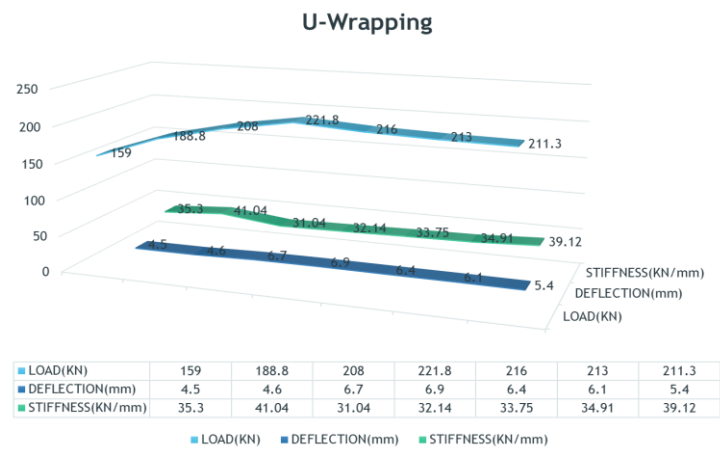
GRAPH 3 LOAD Vs DEFLECTION FOR U-WRAPPING
