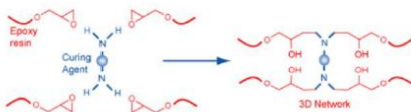
FIG 3 THE CURING OF EPOXY RESIN WITH PRIMARY AMINES
