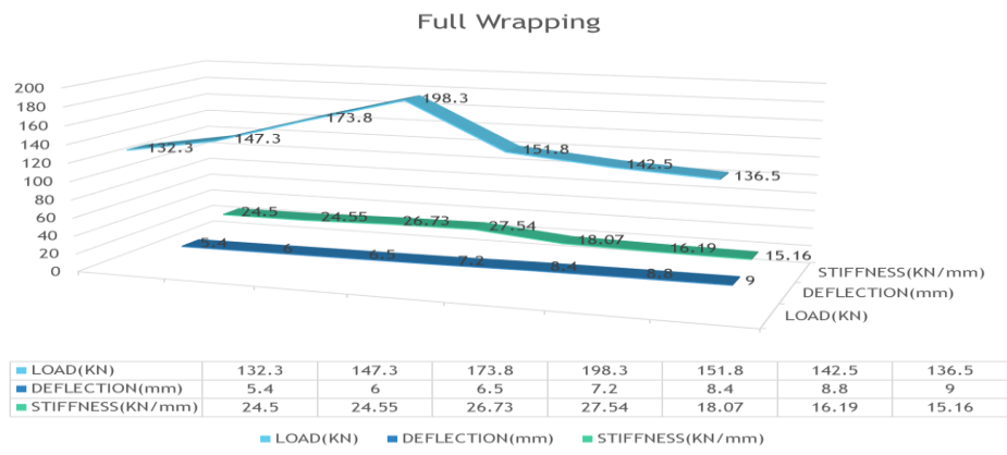
GRAPH 4 LOAD Vs DEFLECTION FOR FULL WRAPPING
