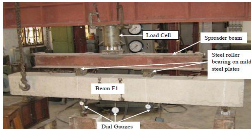
FIG 8 EXPERIMENTAL SETUP FOR TESTING OF BEAMS
