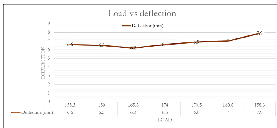
GRAPH 2 LOAD VS DEFLECTION FOR CONTROLLED SHEAR BEAM
