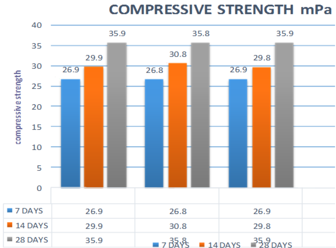
GRAPH 1: COMPRESSIVE STRENGTH (MPA)
