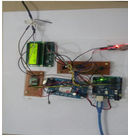
FIG 2. HARDWARE SETUP OF THE SYSTEM
