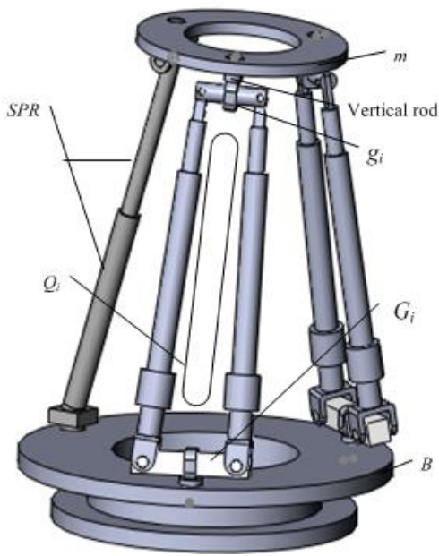
(A) 3D model of the PM with 2Q_i
