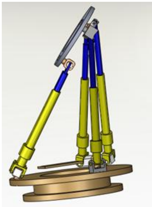
FIGURE 3. THE LOCAL SINGULARITIES OF THE PROPOSED 5-DoF PM
