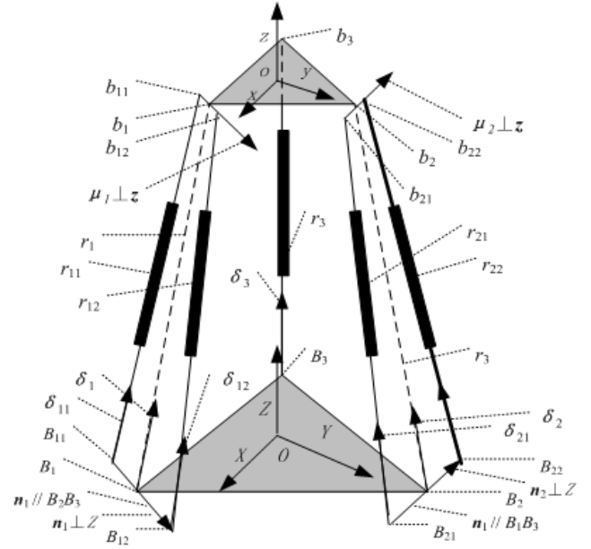
(B) kinematics model of the PM with 2Q_i
