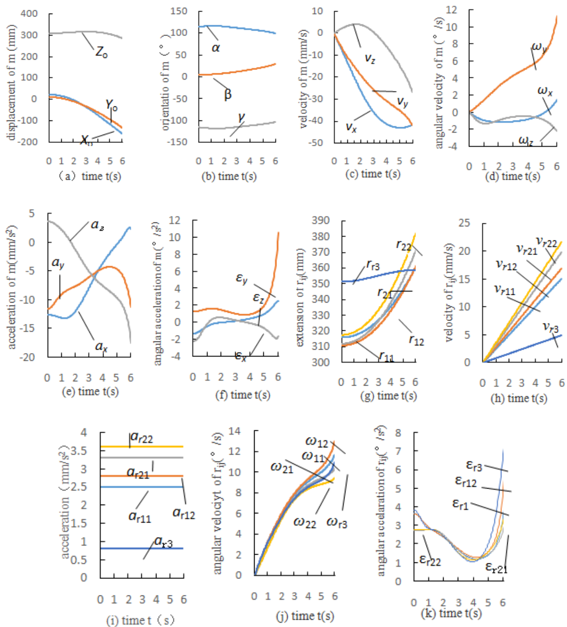
FIGURE 2. ANALYTIC KINEMATICS SOLUTIONS OF THE PM WITH 2 PLANAR LIMBS
