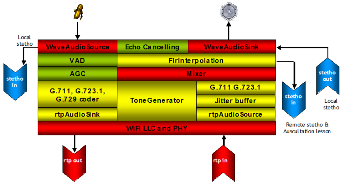
FIGURE 14: SOFTPHONE (MPC) ARCHITECTURE
