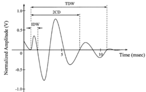
FIGURE 5: NORMALIZED CRACKLE WAVEFORM.
