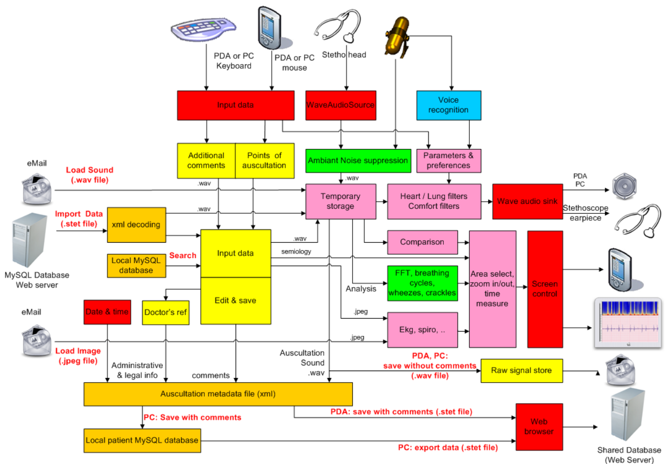
FIGURE 15: eStetho ARCHITECTURE.
