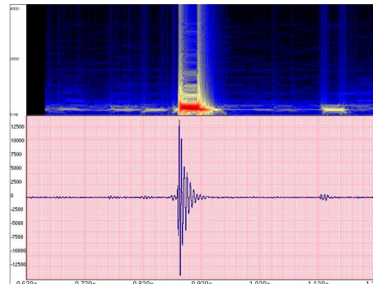
FIGURE 7: ACOUSTIC SIGNATURE OF A CARBON ARTIFICIAL VALVE (SPECIMEN OF SOUND FROM THE ASAP PROJECT).
