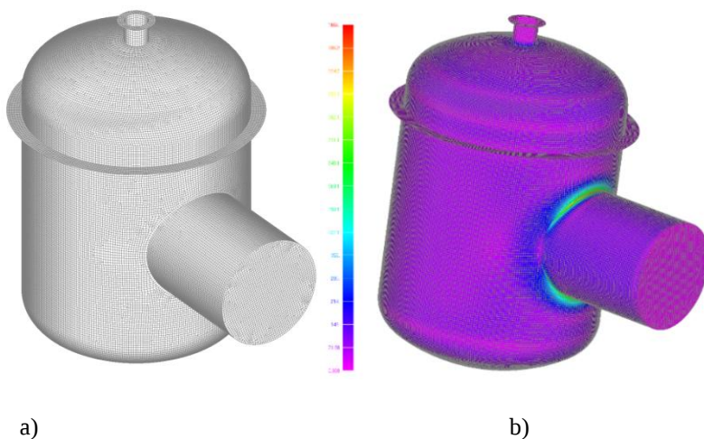
FIGURE A1-1. A) FEM MODEL SHOWING THE ELEMENTS. THERE ARE 63739 ELEMENTS AND 63624 NODES [20]. B) THE MAXIMAL STRESSES ARE AT THE UPPER AND LOWER BRANCH JOINTS
