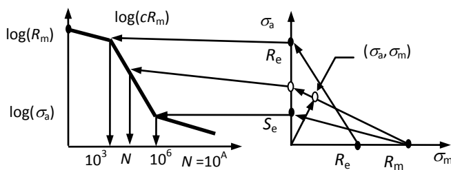
FIGURE 7: THE METHOD OF CALCULATING FATIGUE LIVES OF CRACK INITIATION TIME FROM NORMAL MEAN STRESS AND AMPLITUDE STRESS VS. S-N DIAGRAM
