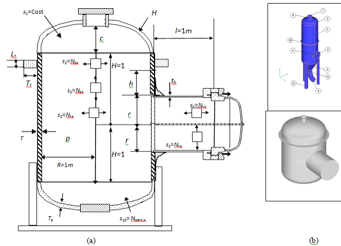
FIGURE 2: A) THE VESSEL IN THIS CASE STUDY. B) A TYPICAL INDUSTRIAL VESSEL AND FEM MODEL IN THIS STUDY.
