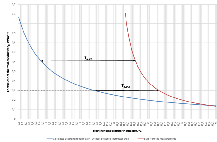
FIG.1. DEPENDENCE OF THERMAL CONDUCTIVITY ON TEMPERATURE THERMISTOR HEATING, BUILT BY THE FORMULA (4) AND ACCORDING TO THE MEASUREMENTS
