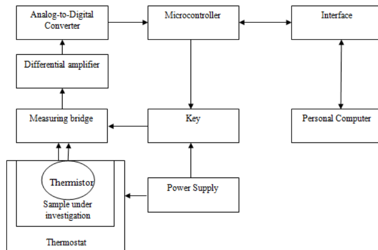
FIG. 3 BLOCK DIAGRAM OF THE DEVICE FOR MEASURING TPC LIQUIDS
