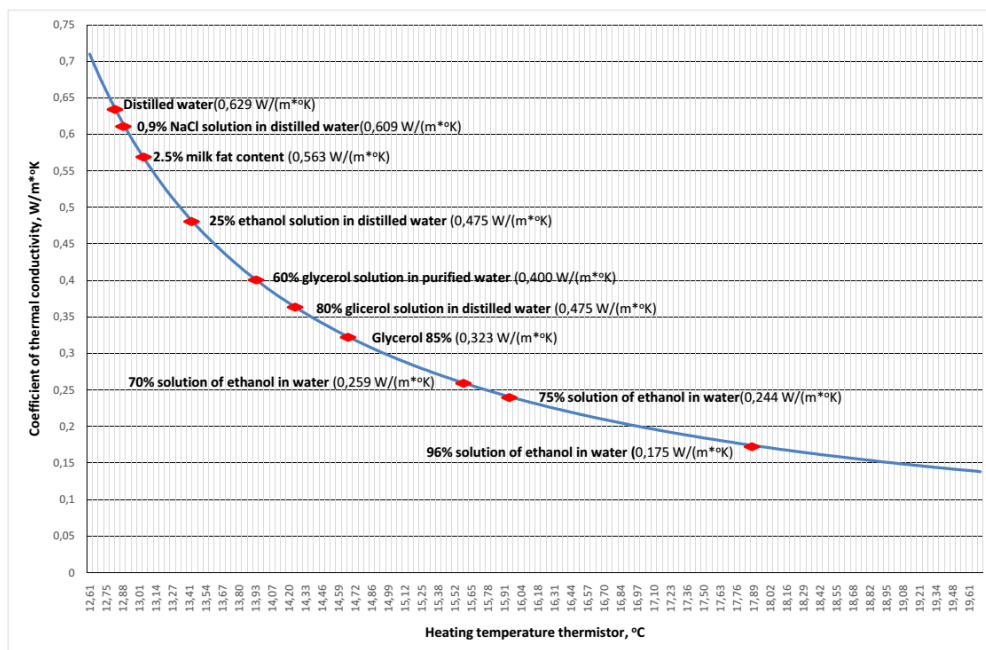
FIG. 5 GRAPH OF THE THERMAL CONDUCTIVITY OF LIQUIDS EXPERIMENTAL HEATING TEMPERATURE THERMISTOR ACCORDING TO MEASUREMENTS AT THE RESEARCH SAMPLE OF +40^{\circ}\text{C}
