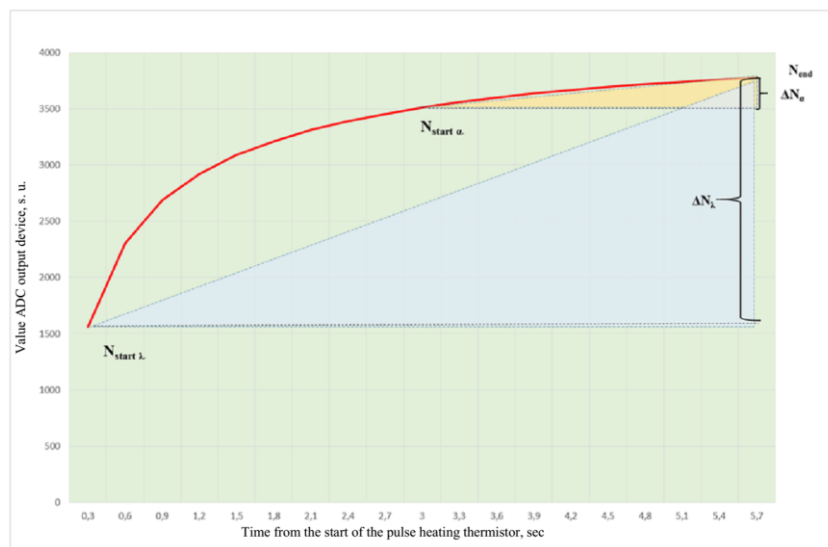
FIG. 4 HEATING THERMOGRAM OF THERMISTOR
