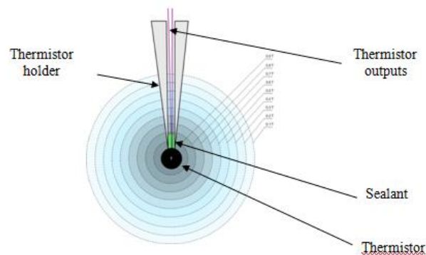
FIG. 2. THE DESIGN OF THE THERMISTOR PROBE TO MEASURE THE THERMAL CONDUCTIVITY OF LIQUIDS
