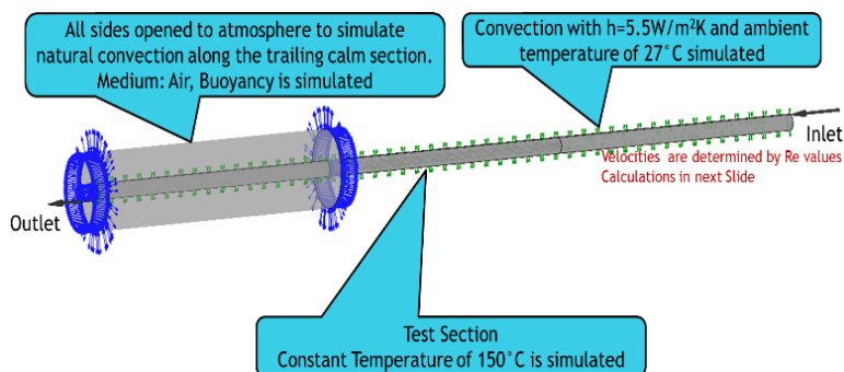
FIG 3: BOUNDARY CONDITIONS
