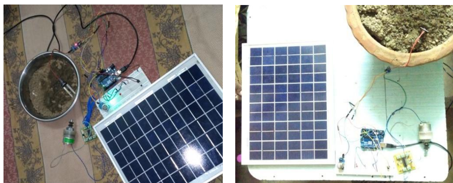
FIG 11. SNAPSHOTS OF AUTOMATIC SOIL MOISTURE MONITORING SYSTEM
