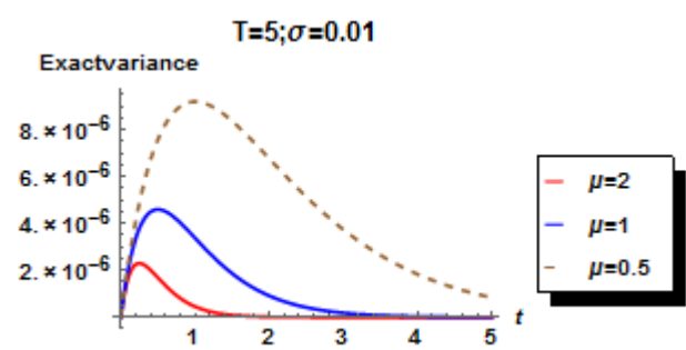
FIG 2. The exact variance at x = \pi / 3 for different values of \mu .
