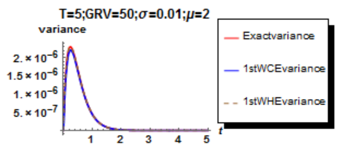
FIG 8. First order response variances for the exact, WCE and WHEP. Comparison between the three variances at x = \pi / 3 .
