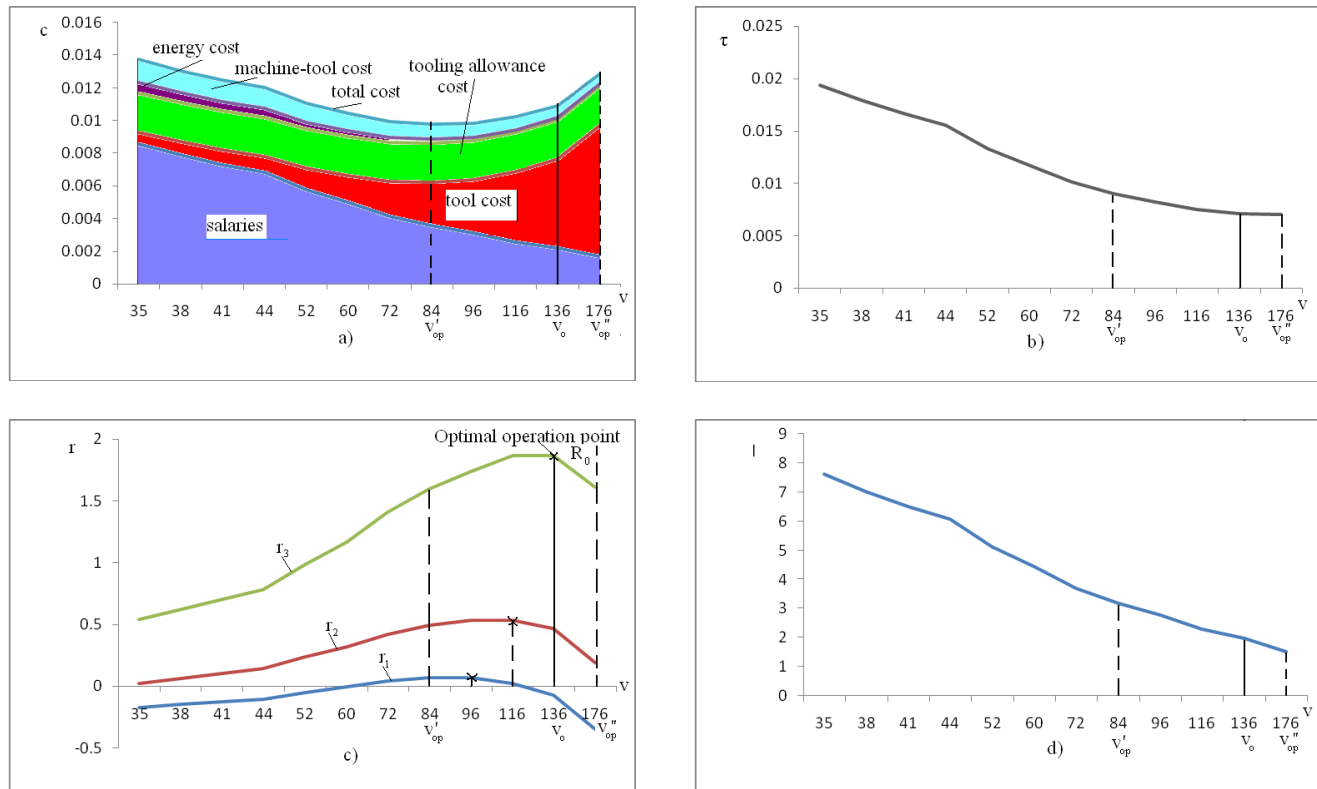
FIG. 3. SIMULATIONS FOR A TURNING PROCESS AND SYSTEM: a) STRUCTURE OF THE COST c ; b) TIME \tau ; c) PROFIT RATE r ; d) ENVIRONMENTAL IMPACT I
