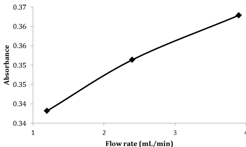
FIGURE 6. EFFECT SAMPLE FLOW RATE ON THE ABSORBANCE SIGNAL
