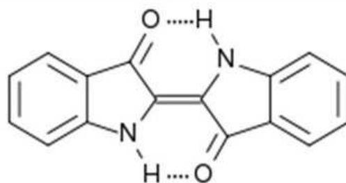
FIGURE 1. CHEMICAL STRUCTURE OF THE REAGENT INDIGO BLUE DYE[12].
