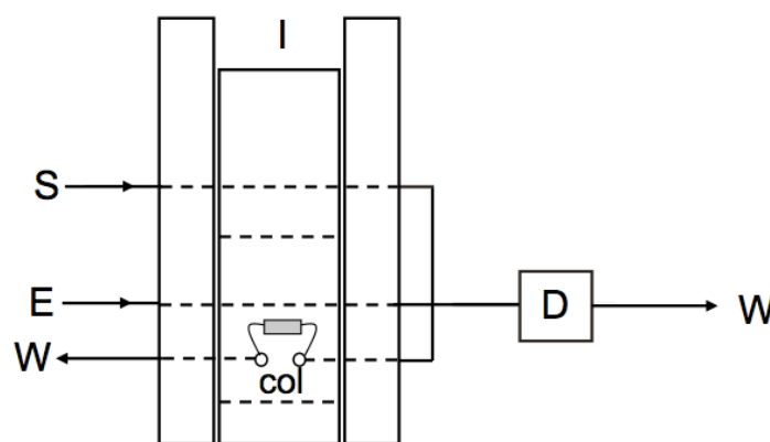
FIGURE 2. FLOW DIAGRAM OF THE SYSTEM FOR 5,5'-DI determination. I: sliding-bar injector, S: sample (2.4 mL min -1 ), E: eluent (3.0 mL min -1 ), col: mini-column (2-mm diameter, 15-mm long, filled with green coconut fiber), D: spectrophotometer (612 nm) and W: waste.
