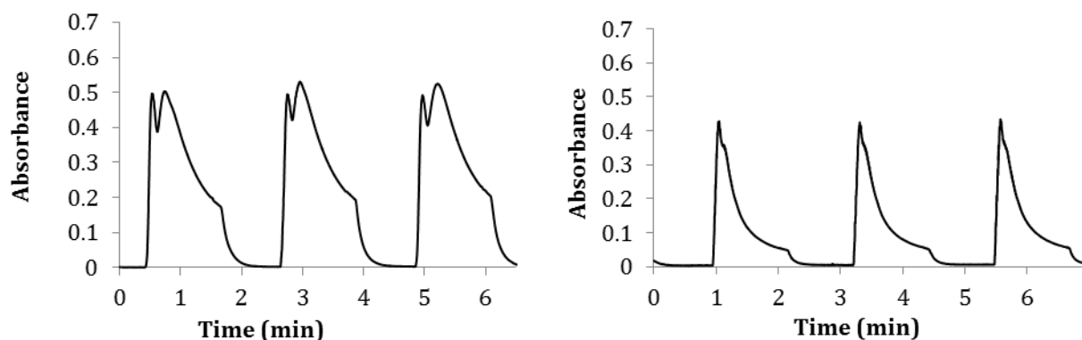
Figure 3. EFFECT OF THE COCONUT FIBER MASS IN THE MINI-COLUMN: (a) 0.0695 g and (b) 0.0211 g using 5,5'-DI solution 3.76 \times 10^{-5} \text{ mol L}^{-1} .
