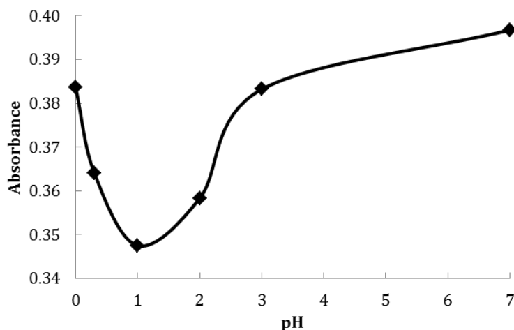
FIGURE 4. INFLUENCE OF THE ELUENT pH ON THE ABSORBANCE.
