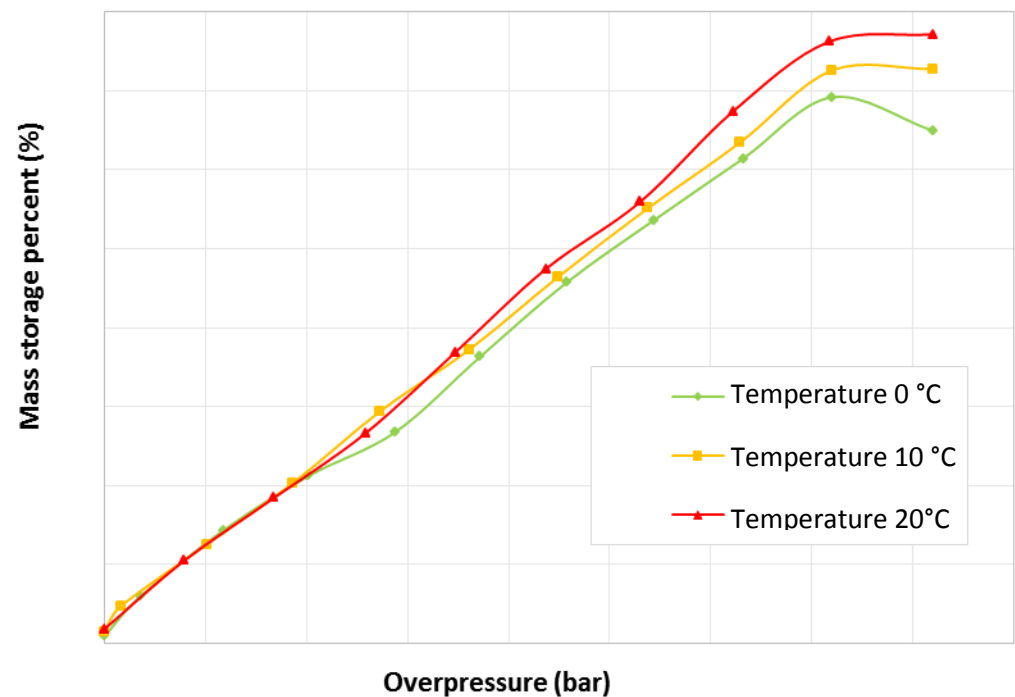
FIG. 8 DEPENDENCE OF MASS STORAGE PERCENT OF GRANULATED ALLOY Ti-Cr-Ni ON OVERPRESSURE FOR DIFFERENT TEMPERATURES (green 0 °C yellow 10 °C red 20 °C)
