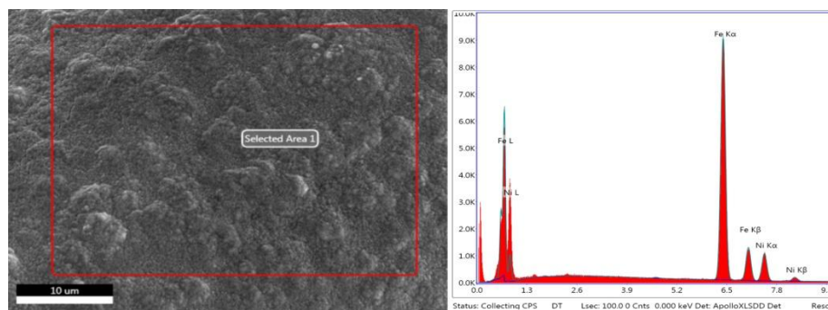
FIGURE 10. SEM AND EDS SPECTRUM OF SAMPLE, 20 MINUTES ELECTRODEPOSITED IN IRON PLATING SOLUTION WITH CURRENT DENSITY 50 A/dm 2 , FOLLOWED BY 1 MINUTE, 2 A/dm 2 , CONCENTRATION RATIO Fe 84.78%, Ni 15.22%.
