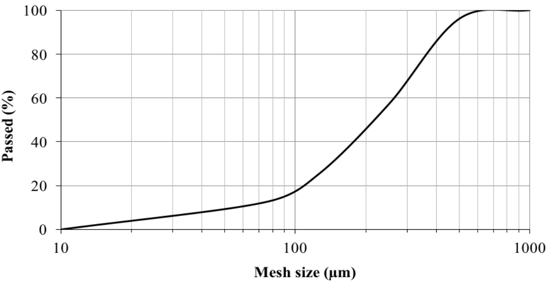
FIGURE 3. SIEVE ANALYSIS FOR THE BA 2
