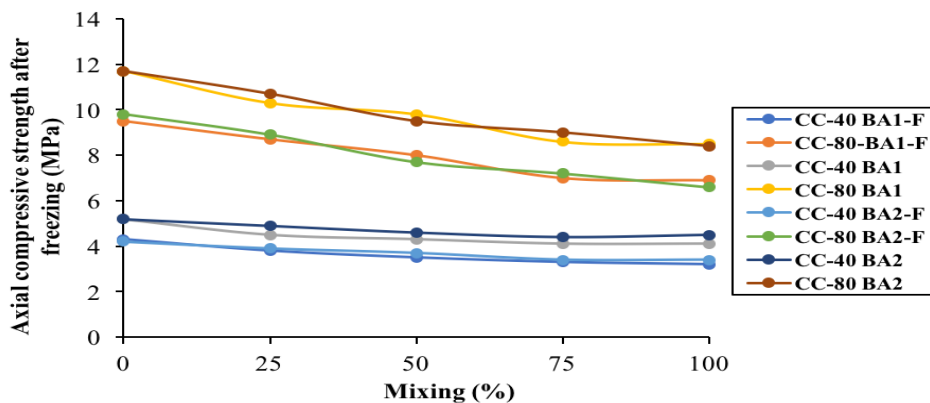
FIGURE 8. ACCORDING TO MIXING RATIOS, AXIAL COMPRESSIVE STRENGTH VALUES OF THE SAMPLES AFTER FREEZING (F: FROZEN)
