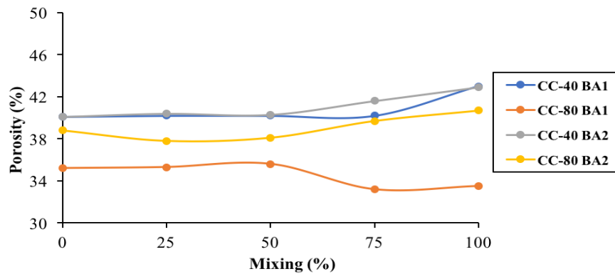
FIGURE 7. ACCORDING TO MIXING RATIOS, POROSITY VALUES OF THE SAMPLES
