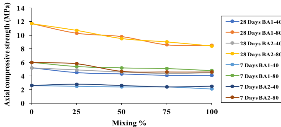
FIGURE 4. ACCORDING TO MIXING RATIOS, AXIAL COMPRESSIVE STRENGTH VALUES OF THE SAMPLES
