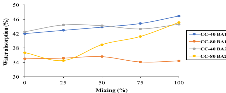
FIGURE 6. ACCORDING TO MIXING RATIOS, WATER ABSORPTION PERCENTAGE VALUES OF THE SAMPLES
