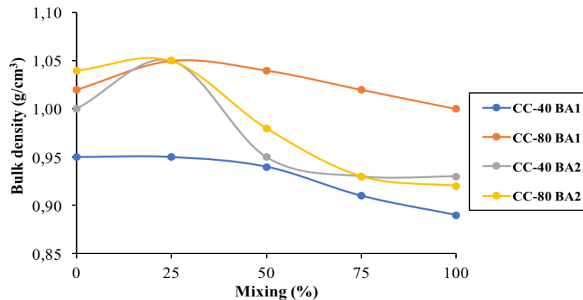
FIGURE 5. ACCORDING TO MIXING RATIOS, BULK DENSITY VALUES OF THE SAMPLES
