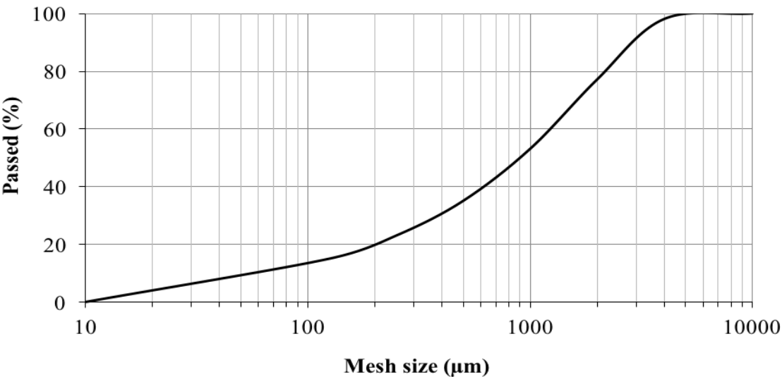
FIGURE 1. SIEVE ANALYSIS FOR THE PUMICE
