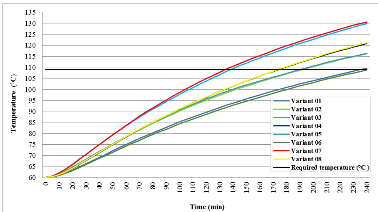
FIG. 10 COURSE OF TEMPERATURE IN THE STATOR FOR INDIVIDUAL VARIANTS (TIME VERSUS TEMPERATURE)
