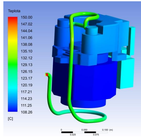
FIG. 12 TEMPERATURE ON THE STRUCTURE UNDER CURRENT CONDITIONS AFTER 240 MINUTES
