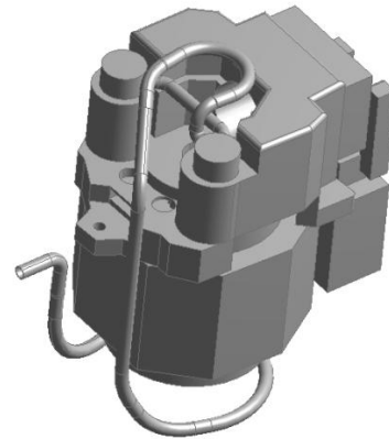
FIG. 8 SIMPLIFIED GEOMETRY OF THE COMPLETE COMPRESSOR WITHOUT COVER
