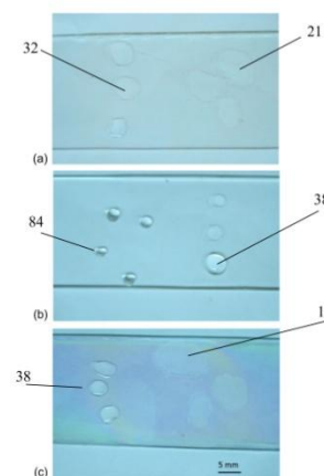
FIG. 4. WATER DROPS ON SILICATE GLASS (A), PMMA (B) AND \text{TiO}_2 FILM (ANATAZE) (C): LEFT – BEFORE UV IRRADIATION, RIGHT – AFTER UV IRRADIATION. NUMBERS SHOW CONTACT ANGLE IN DEG. CALCULATED FROM EQ. (1a)
