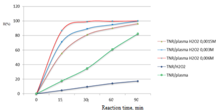
FIG. 5. TNR DEGRADATION EFFICIENCY BY PLASMA COMBINED WITH H 2 O 2
