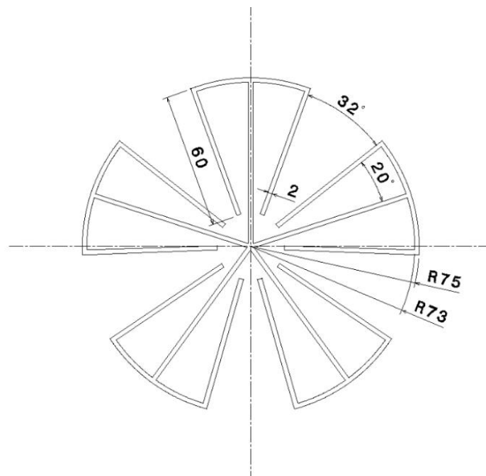
FIGURE 3: Design of internal heat transfer intensifier
