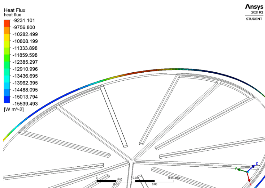
FIGURE 6: Heat removal by cooling
