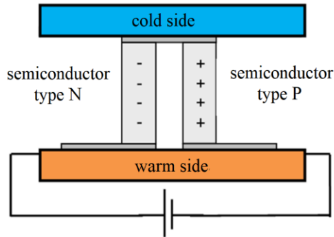
FIGURE 1: One thermoelectric cell
