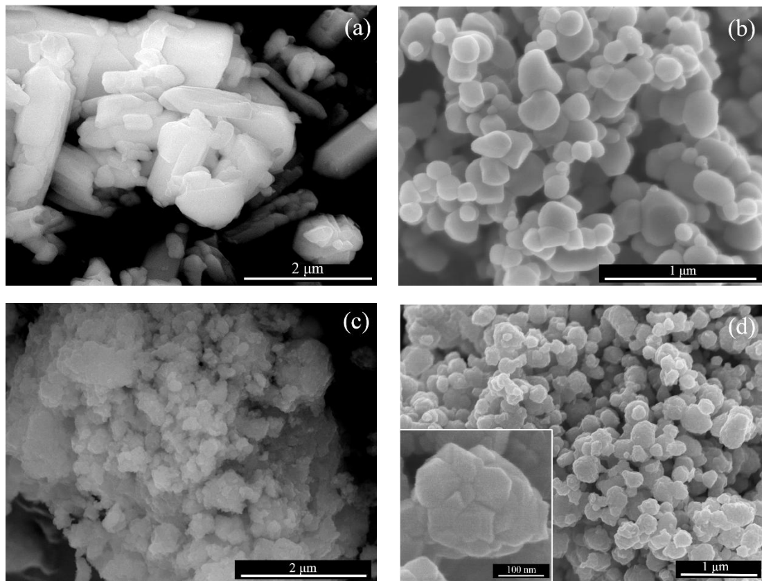
FIG 6: SEM MICROGRAPHS OF: (A) COMMERCIAL BC AND (B) \text{TiO}_2 , (C) AS MILLED MIXTURE BC AND \text{TiO}_2 AND (D) BT POWDERS DERIVED FROM CALCINATION AT 900°C FOR 6H.
