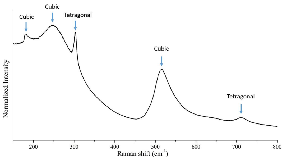
FIG 5: RAMAN SPECTRUM OF \text{BaTiO}_3 POWDERS (OBTAINED BY 8H OF MILLING AT 350\text{ RPM} , AND CALCINATED FOR 6H AT 900^\circ\text{C} ).
