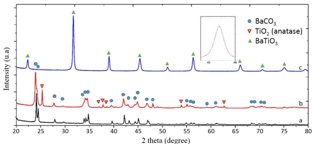
FIG 4: XRD PATTERNS OF POWDERS: (A) COMMERCIAL BC AND THE 8H MILLED MIXTURE BC AND \text{TiO}_2 BEFORE (B) AND (C) AFTER CALCINATION (FOR 6H AT 900^\circ\text{C} ).
