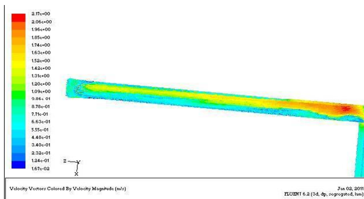
FIGURE 3. PATTERN OF FLOW FIELD VELOCITY VECTOR
