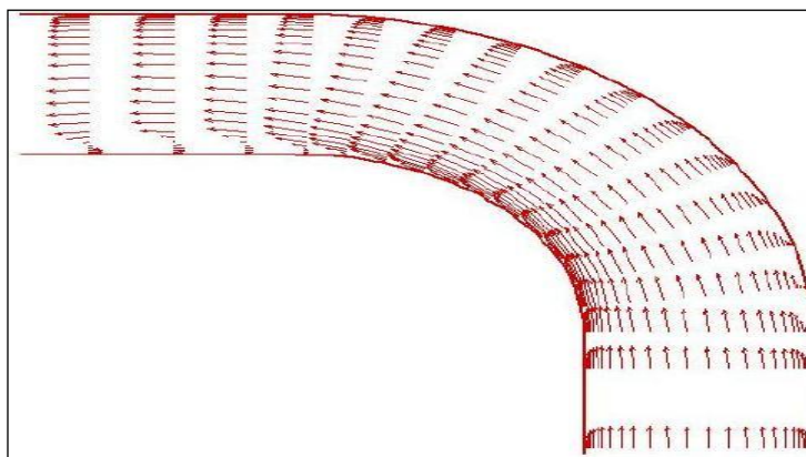
FIGURE 4. FLOW FIELD VELOCITY VECTOR DISTRIBUTION
