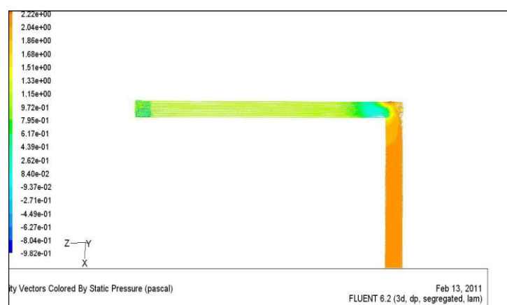
FIGURE 2. PATTERN OF FLOW FIELD PRESSURE VECTOR
