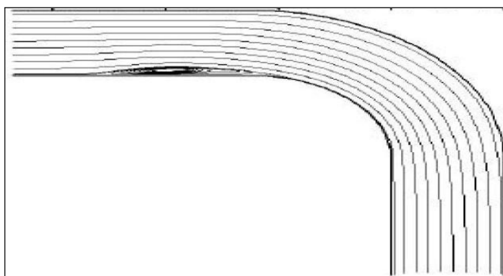
FIGURE 5. CURVED TUBE VORTEX DISTRIBUTION
