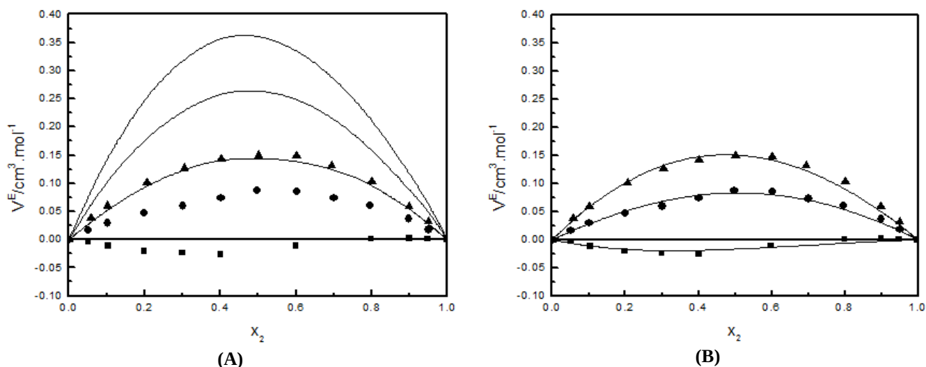
FIGURE 2. COMPARISON BETWEEN EXPERIMENTAL (SYMBOLS) AND MODELING (LINES) EXCESS MOLAR VOLUME FOR 1,2-DIMETHYLBENZENE (1) WITH ALKANES (2) BINARY MIXTURES: OCTANE (■), NONANE (●) OR DECANE (▲) AT 298.15 K. A) NITTA-CHAO PREDICTIONS AND (B) ERAS CORRELATIONS.
