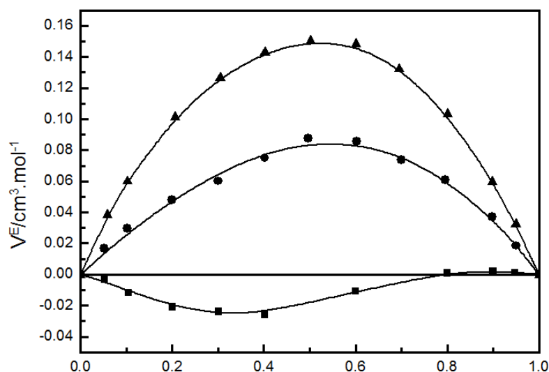
FIGURE 1. EXPERIMENTAL (SYMBOLS) AND REDLICH-KISTER (LINES) CORRELATION FOR THE EXCESS MOLAR VOLUME AT 298.15 FOR 1,2-DIMETHYLBENZENE (1) WITH ALKANES (2) BINARY MIXTURES: OCTANE (■), NONANE(●) AND DECANE(▲).
