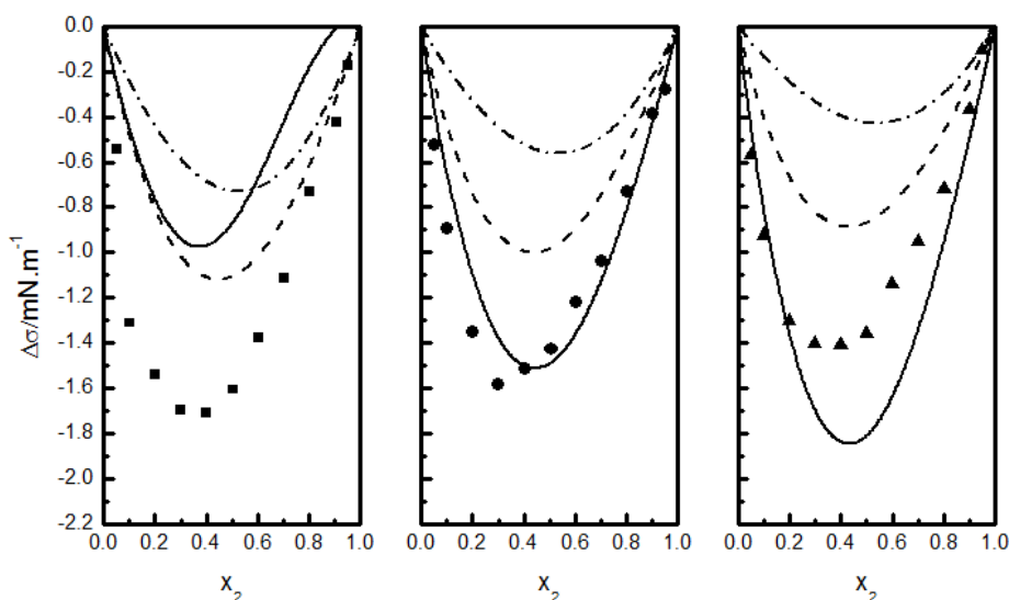
FIGURE 6: COMPARISON BETWEEN EXPERIMENTAL (SYMBOLS) AND MODELING RESULTS (LINES) FOR THE DEVIATION SURFACE TENSION AT 298.15 K IN 1,2-DIMETHYLBENZENE (1) WITH ALKANES (2) BINARY MIXTURES: OCTANE ( \blacksquare ), NONANE ( \bullet ) AND DECANE ( \blacktriangle ). THE LINES ARE: SE (—); HSEG (---); HSIS (-.-.) MODELS.
