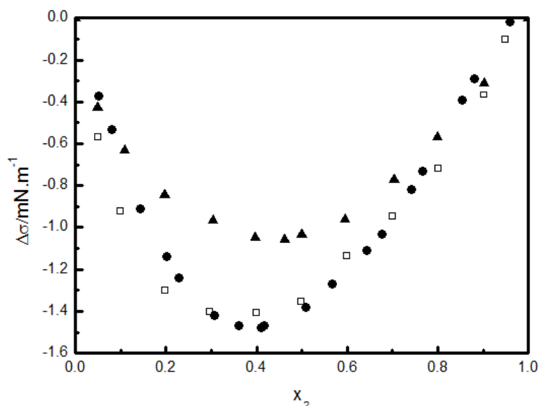
FIGURE 5. EXPERIMENTAL SURFACE TENSION DEVIATION OF DIMETHYLBENZENE ISOMERS (1) + ALKANES (2): 1,2-DIMETHYLBENZENE + DECANE ( \square ) (THIS WORK), 1,4-DIMETHYLBENZENE + DECANE ( \blacktriangle ) [18] AND 1,3-DIMETHYLBENZENE + HEXANE AT 298.15K ( \bullet ) [37].
