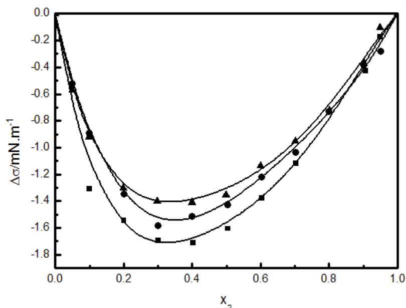
FIGURE 4. EXPERIMENTAL (SYMBOLS) AND REDLICH-KISTER (LINES) CORRELATION FOR THE DEVIATION SURFACE TENSION AT 298.15 K FOR 1,2-DIMETHYLBENZENE (1) WITH ALKANES (2) BINARY MIXTURES: OCTANE (■), NONANE(●) AND DECANE(▲).
