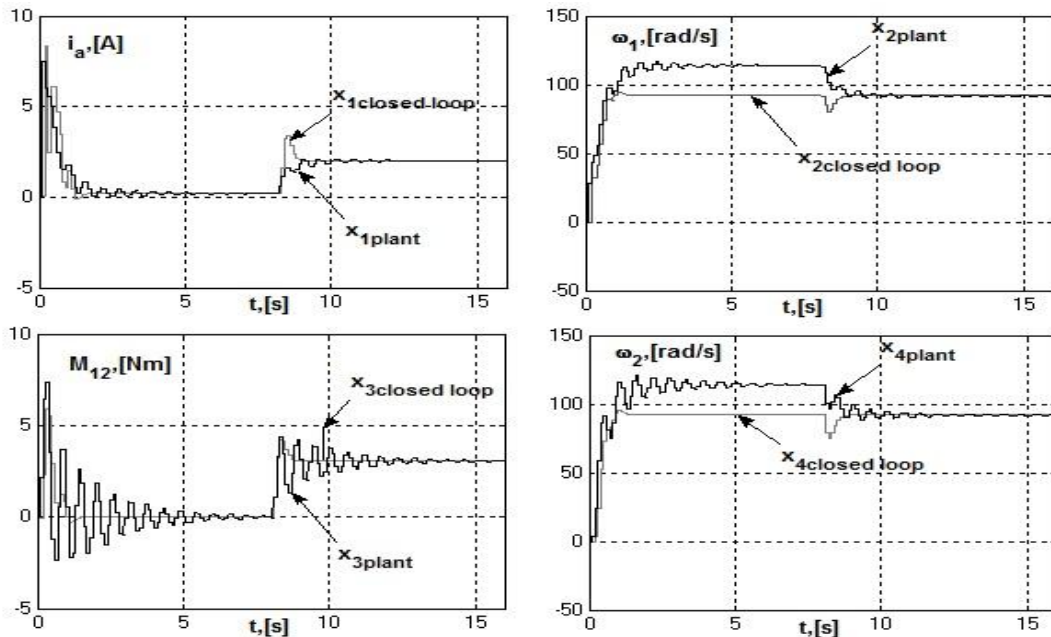
FIGURE 3. PLANT AND CLOSE-LOOP STATE VARIABLE START PROCESSES
