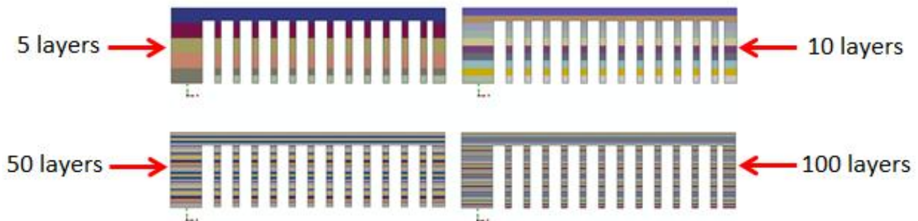
FIGURE 6: FE-MODELS WITH DIFFERENT SEQUENTIAL NUMBER OF LAYER ACTIVATION STEPS
