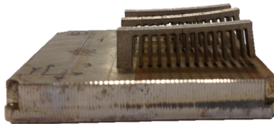
FIGURE 3: SUPPORT CUTTING FROM THE BASE PLATE BY EDM AND RESULTING DISTORTION
