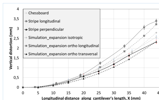
FIGURE 12: COMPARISON OF EXPERIMENTAL VS SIMULATION DISTORTIONS WITH DIFFERENT THERMAL EXPANSION COEFFICIENTS (ISOTROPIC AND ORTHOTROPIC)
