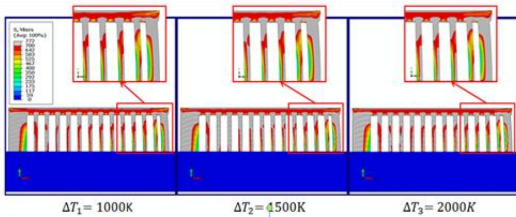
FIGURE 11: RESIDUAL STRESSES BEFORE CUTTING PROCESS PREDICTED BY ISOTROPIC NUMERICAL MODEL FOR DIFFERENT INITIAL TEMPERATURES.
