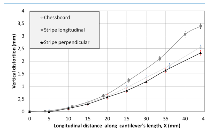
FIGURE 7: EXPERIMENTALLY MEASURED VERTICAL DISTORTION OF CANTILEVER SPECIMENS MANUFACTURED WITH DIFFERENT SCANNING STRATEGIES.
