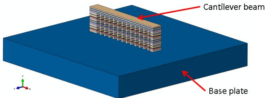
FIGURE 5: FE-MODEL OF CANTILEVER SAMPLE
