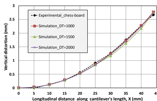
FIGURE 10: COMPARISON OF PREDICTED VERTICAL DISTORTION ALONG CANTILEVER LENGTH AFTER INTRODUCING DIFFERENT INITIAL TEMPERATURES.
