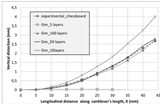
FIGURE 8: COMPARISON OF PREDICTED VERTICAL DISTORTION ALONG CANTILEVER LENGTH WITH EXPERIMENTAL MEASUREMENTS (CHESS-BOARD SCANNING STRATEGY)
