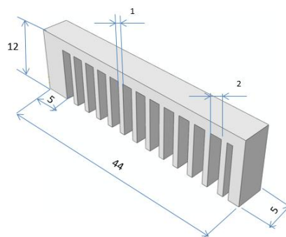
FIGURE 1: CANTILEVER SHAPE SPECIMEN WITH DIMENSIONS (MM)
