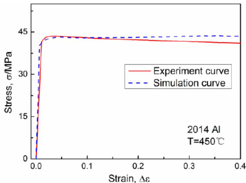
FIGURE 3 FEM-SIMULATED AND EXPERIMENTAL STRESS–STRAIN CURVES DURING THE FIRST MDF PASS OF 2014 ALUMINUM ALLOYS AT 450°C AND AT A DEFORMATION SPEED OF 0.15 \text{mm s}^{-1}
