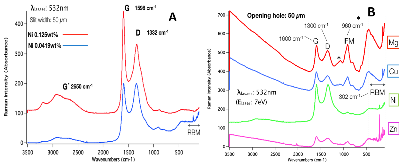
FIG. 5. Raman spectra of thin films: a) comparison of NiPc composites at different concentrations; b) comparison of samples obtained by pyrolysis using different MPc at 0.5 wt. %. (RBM is Radial Breathing Mode 140 \leq \nu \leq 350 \text{ cm}^{-1} ) and IFM (intermediate frequency modes \text{IFM}^- = 750 \text{ cm}^{-1} , \text{IFM}^+ = 960 \text{ cm}^{-1} ). The features marked with '*' at 248, 521 and 962 \text{ cm}^{-1} are from the Si/SiO 2 substrate and are used for calibration of the nanotube Raman spectrum [29]).
