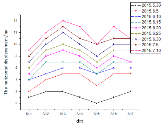
FIGURE 7. THE HORIZONTAL DISPLACEMENT OF DIFFERENT TIME S11~S17
