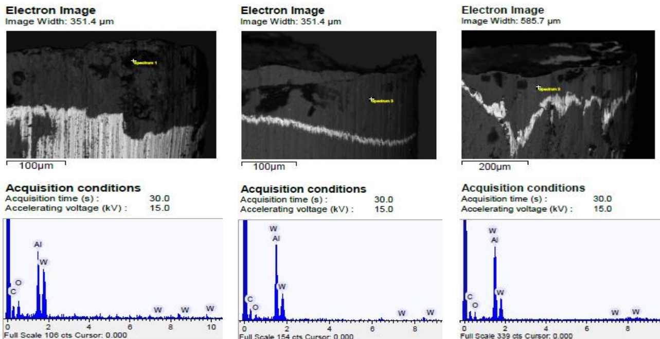
(a) 1.0 mm nozzle orifice
