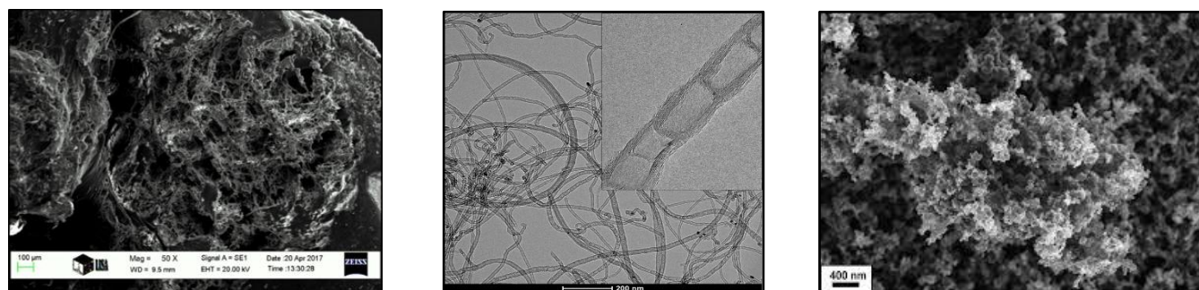
FIG. 1. SEM-Image of raw caoutchouc (50x magnification), CNT and Soot
