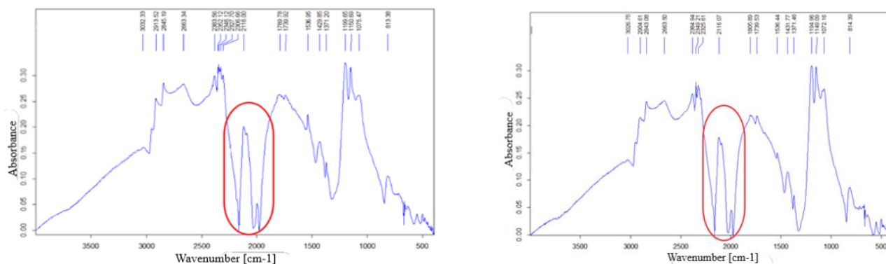
FIG. 5. Absorbance wave number of soot-cured,(a), nanotube-cured (b) vulcanised specimen before aging
