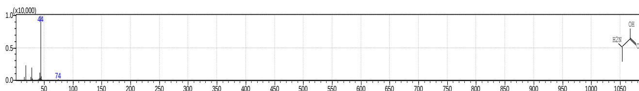
FIGURE 4: Mass spectrum detected by GC-MS of Alanine.
