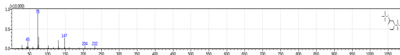
FIGURE 5: Mass spectrum detected by GC-MS of Glycine, N-formyl-N-(trimethylsilyl)-, trimethylsilyl ester.
